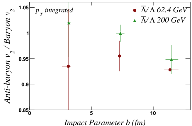
FIG. 4: (color online). The p_T integrated ratio of \bar{\Lambda} v_2 to \Lambda v_2 for three centrality intervals: 0%–10%, 10%–40%, and 40%–80%. The data are from Au+Au collisions at \sqrt{s_{NN}} = 62.4 and 200 GeV.
