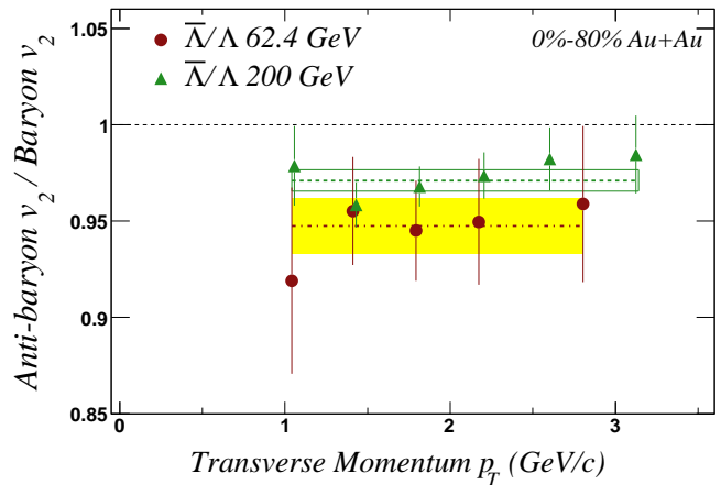
FIG. 3: (color online). The ratio of \bar{\Lambda} v_2 to \Lambda v_2 . The data are from minimum bias Au+Au collisions at \sqrt{s_{NN}} = 62.4 and 200 GeV. The bands show the average values of the ratios within the indicated p_T ranges.
