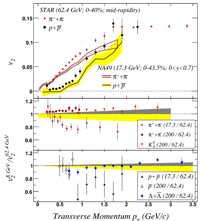
FIG. 8: (color online). Top panel: v_2 for pions and protons at \sqrt{s_{NN}} = 62.4 and 17.3 GeV. The 62.4 GeV data are from TOF and dE/dx measurements combined. Middle and bottom panel: ratios of v_2 for \pi^+ + \pi^- , K_S^0 , p + \bar{p} , \Lambda + \bar{\Lambda} and at different center-of-mass energies scaled by the values at 62.4 GeV. The grey and yellow bands represent systematic uncertainties in the v_2 ratios arising from non-flow effects. The grey bands (above unity) are the uncertainties for the 200 GeV/62.4 GeV data and the yellow bands (below unity) are for the 17.3 GeV/62.4 GeV data.
