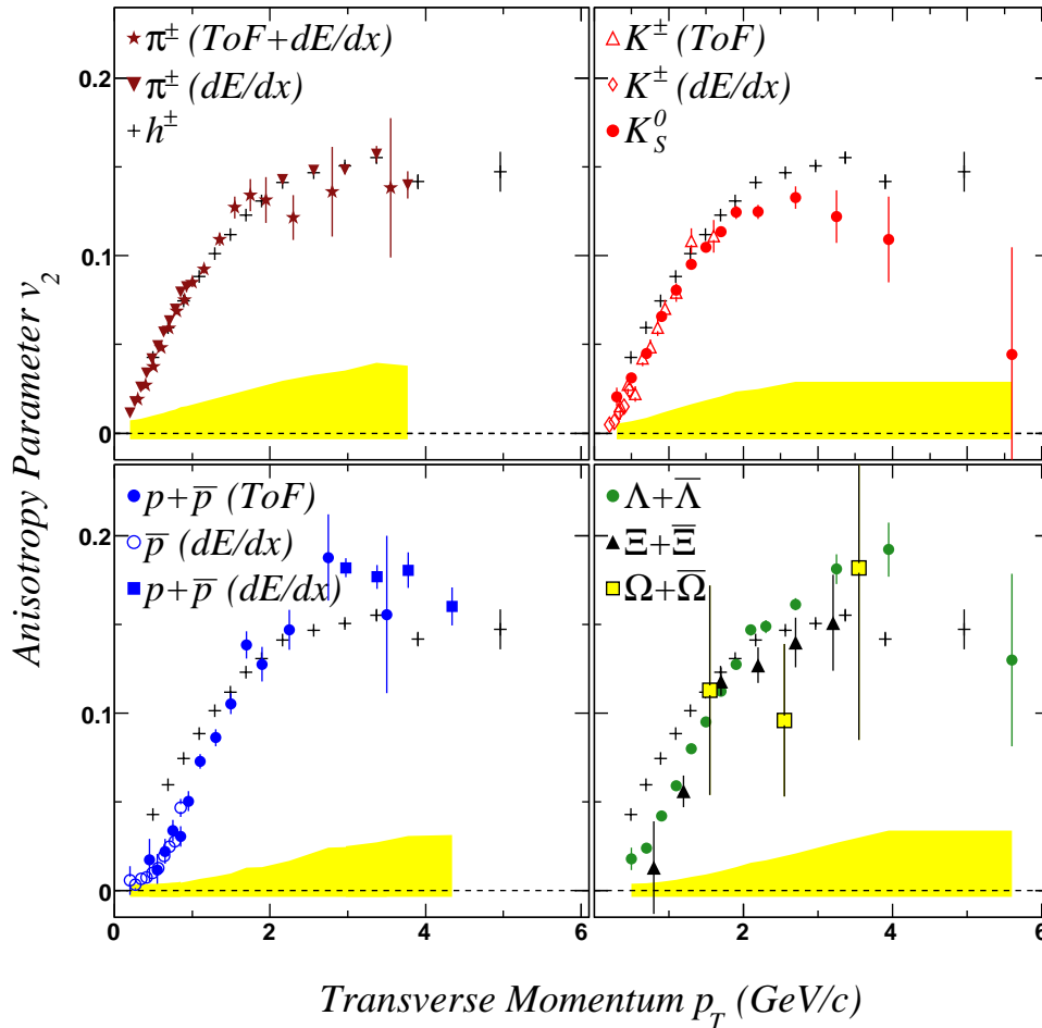
FIG. 1: (color online). Minimum-bias (0–80% of the collision cross section) v_2(p_T) for identified hadrons at |\eta| < 1 from Au+Au collisions at \sqrt{s_{NN}} = 62.4 GeV. To facilitate comparisons between panels, v_2 values for inclusive charged hadrons are displayed in each panel. The error bars on the data points represent statistical uncertainties. Systematic uncertainties for the identified particles are shown as shaded bands around v_2 = 0 .
