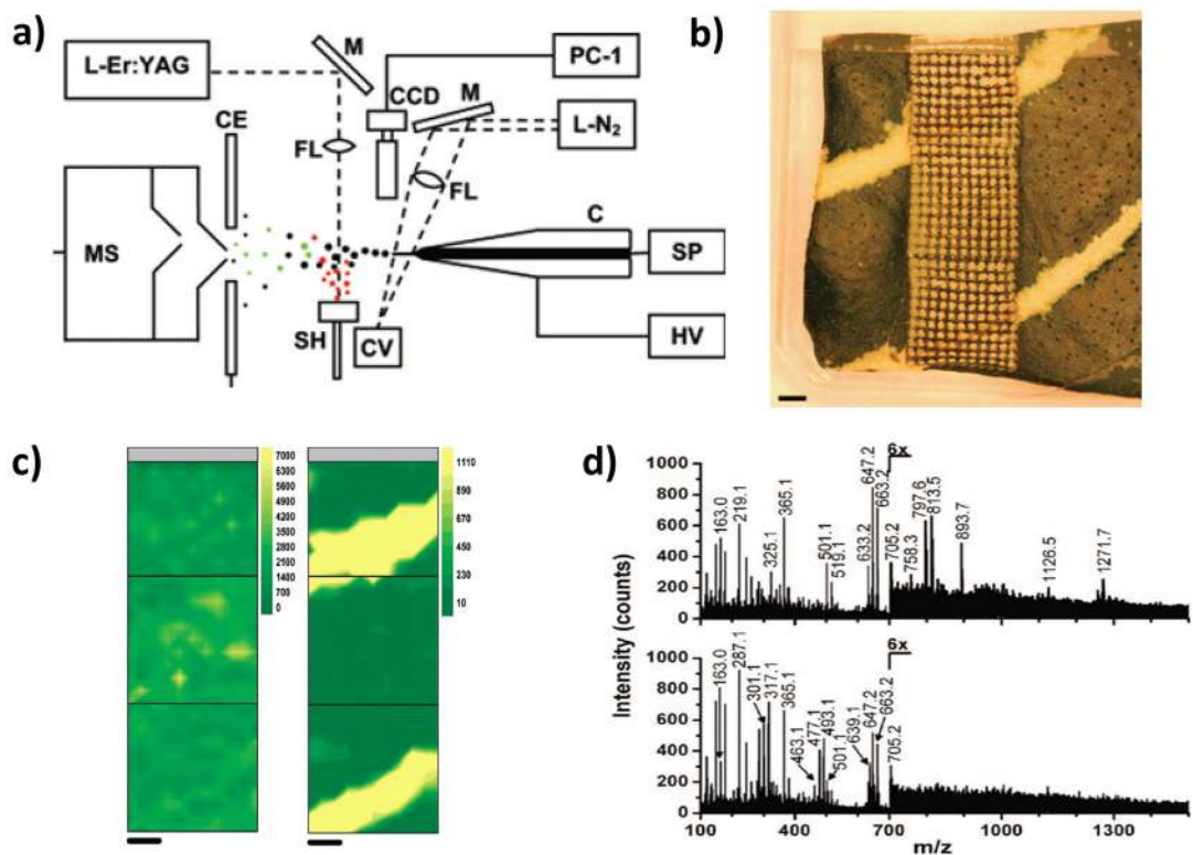
Figure 4. LAESI MS imaging (a) Schematic diagram of the LAESI instrumentation. (C, capillary; SP, syringe pump; HV, high-voltage power supply; L-N 2 , nitrogen laser; M, mirrors; FL, focusing lenses; CV, cuvette; CCD, CCD camera with short-distance microscope; CE, counter electrode; OSC, digital oscilloscope; SH, sample holder; L-Er:YAG, Er:YAG laser; MS, mass spectrometer; PC-1 to PC-3, personal computers). (b) Variegated A. squarrosa leaf probed with LAESI-MS while rastering the surface with a focused infrared laser beam over three adjacent 4 mm by 4 mm areas. The live tissue surface was ablated from a circular area (350- \mu m diameter) with a 400- \mu m step size. (c) Contour plots show the distribution of ions detected at m/z 663 and m/z 493, respectively. (d) Mass spectra obtained at different regions of the leaf (top: green sectors, bottom: yellow sectors). Length scale bars correspond to 1 mm. Panel a is reproduced from (Nemes & Vertes, 2007) with permission. Panels b–d are reproduced from (Nemes, et al., 2008) with permissions.
