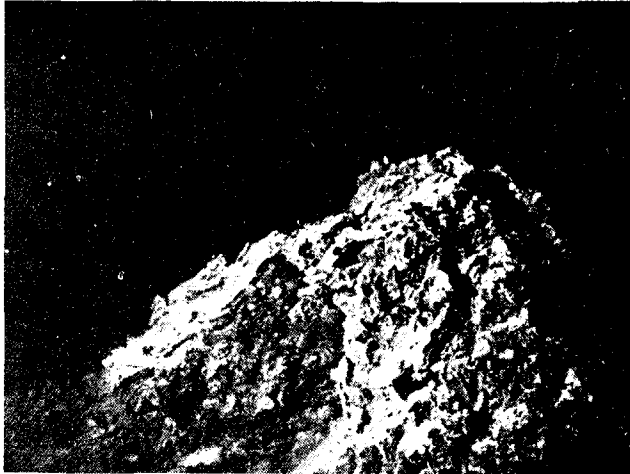
Fig. 3 Photograph of a variegated hornito-like edifice taken during dive CY 78-06. The diameter of the edifice is ~2 m. A second edifice can be seen in the background.
