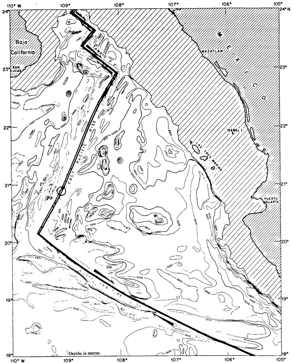
Fig. 1 Setting of the axial zone of the East Pacific Rise where the sulphide ore deposits were explored and sampled (circle).
