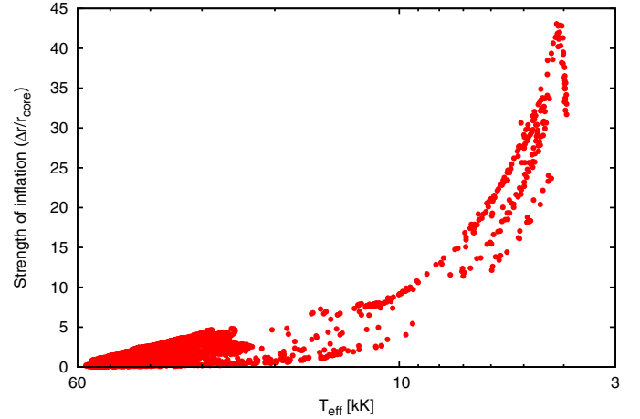
Fig. 11. Inflation as a function of the effective temperature for all analysed models that fulfill our inflation criterion.
