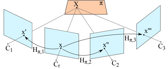
Figure 4: Multi-view setup with four cameras and homographies from reference camera C_r to three other cameras.
