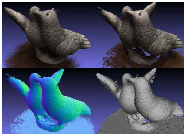
Figure 1: Results on one of the 80 evaluated objects on the DTU benchmark [22]. Top left : Ground truth point cloud; top right : reconstructed point cloud with texture; bottom left : color-coded surface normals; bottom right : reconstructed surface.
