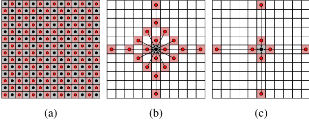
Figure 2: The propagation scheme: (a) Depth and normal are updated in parallel for all red pixels, using black pixels as candidates, and vice versa. (b) Planes from a local neighborhood (red points) serve as candidates to update a given pixel (black). (c) Modified scheme for speed setting, using only inner and outermost pixels of the pattern.
