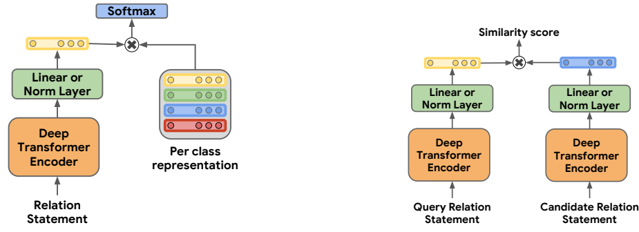
Figure 2: Illustration of losses used in our models. The left figure depicts a model suitable for supervised training, where the model is expected to classify over a predefined dictionary of relation types. The figure on the right depicts a pairwise similarity loss used for few-shot classification task.
