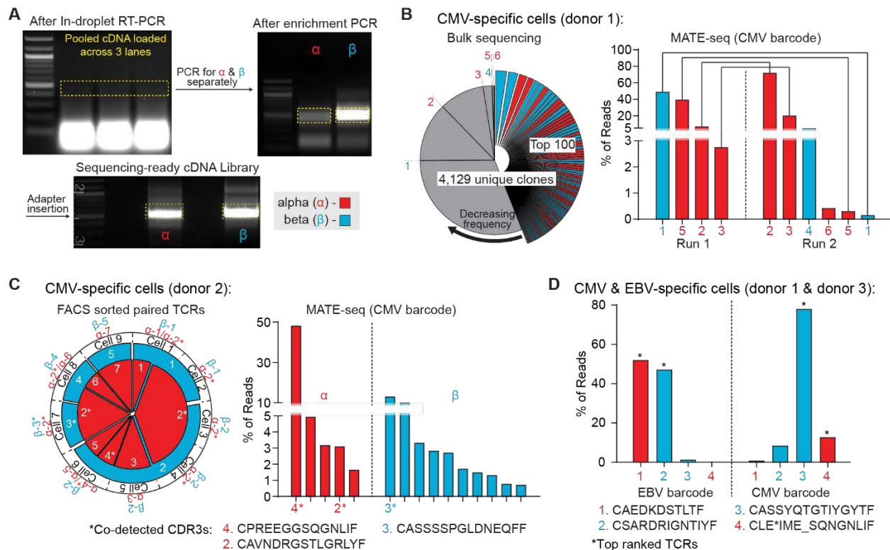
Figure 3: MATE-seq sequencing results. (A) After microfluidic processing, the RT-PCR product was purified and modified with two PCR steps to generate a sequencing-ready library. Gel ladder is 100 base pairs. (B) The bulk analysis of cells containing CMV-specific cells (donor 1) yielded 4,129 sequenced TCR clones, with no single TCR contributing more than 3% of total reads. Two independent MATE-seq analyses of the same cells yielded 2 unique TCR \beta chains and 4 unique TCR \alpha chains, all of which were only associated with CMV barcodes, with 1 \beta and 3 \alpha chains shared across both runs. While these 6 CDR3s contributed to >99% of total reads in MATE-seq, they only represented 0.09% of total reads from bulk sequencing. (C) FACS sorting and sequencing of a different set of CMV-specific T-cells (donor 2) yield 9 paired TCRs, with the most common \alpha and \beta chains appearing in 6 and 4 cells, respectively. MATE-seq analysis of the same cells co-detected 3 of the same CDR3s, one of which was the most common \alpha chain from FACS analysis. (D) Multiplexed MATE-seq of CMV and EBV-specific cells (mixture of donor 1 and 3) revealed dominant TCR \alpha and \beta chains for each antigen.
