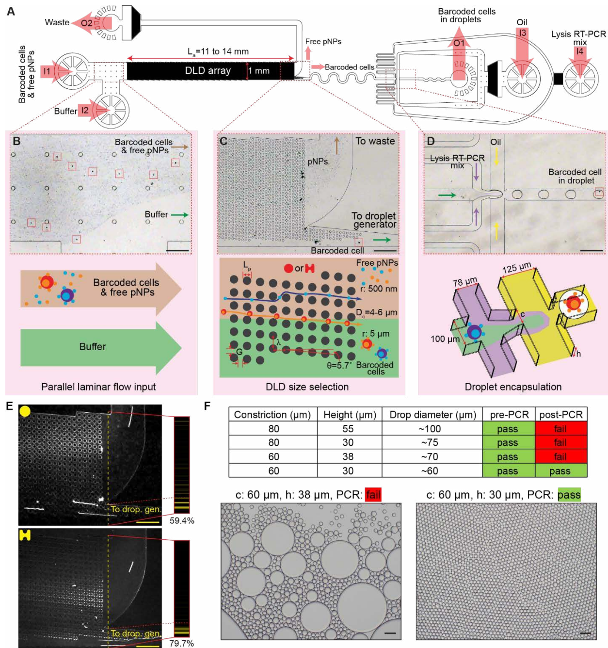
Figure 2: Microfluidic device for MATE-seq. (A) The device integrates a DLD array on the front end of a droplet generator, and features 4 inputs (I1 to I4) for barcoded cells-free pNPs mixture, buffer, encapsulation oil, and lysis/RT-PCR mix, as well as 2 outputs (O1 and O2) for the water-in-oil droplets created by the droplet generator and waste. (B) The barcoded cells and free pNPs are flowed in parallel with buffer optimized for RT-PCR with minimal mixing by diffusion. (C) After DLD processing, the barcoded cells are displaced into the buffer stream toward the droplet generator, with full removal of free pNPs into the waste. The physical dimensions of the DLD array determine a critical sorting diameter, D_c . (D) Barcoded cells are encapsulated in water-in-oil droplets with lysis RT-PCR mixture, and collected for
