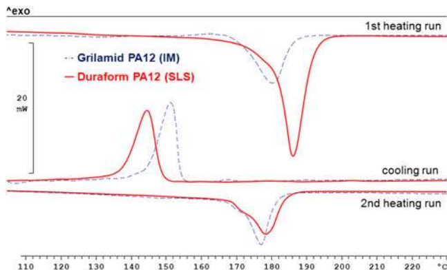
FIG. 5. Comparison of a commercial (Grilamid) and a SLS (Duraform PA) polyamide 12; enlargement of sintering window.
