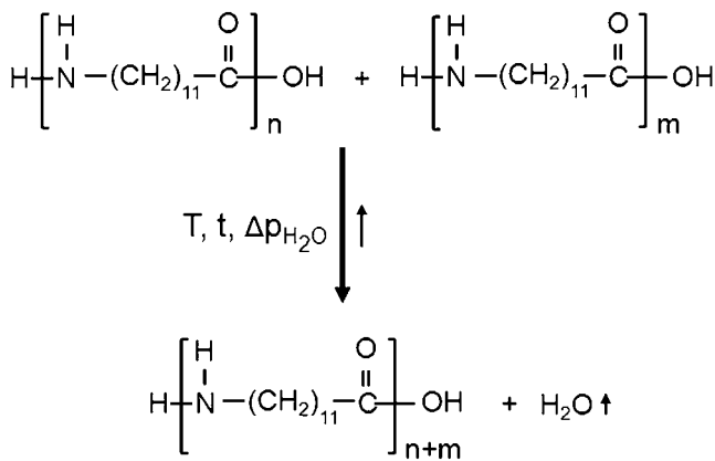
FIG. 10. Nature of solid state condensation in polyamide 12.
