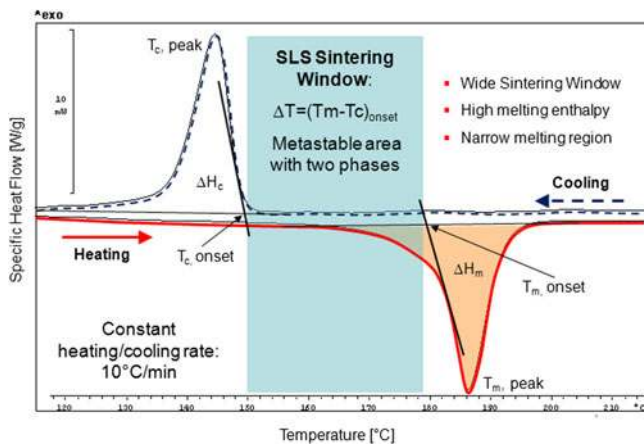
FIG. 2. DSC-Thermogram indicating the ‘sintering window’ of SLS-processing - region between melting ( T_m ) and crystallisation ( T_c ).
