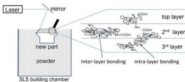
FIG. 12. Interlayer reaction of polyamide 12 during SLS processing.
