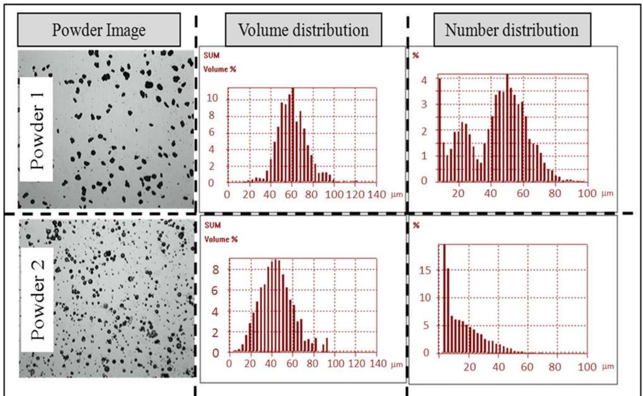
FIG. 4. Distribution of powders with similar volume distribution and dissimilar number distribution.
