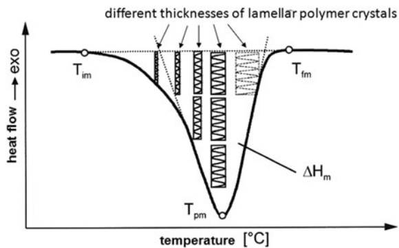
FIG. 6. Nature of broad melting points of polymers; different thickness of lamellar crystals.
