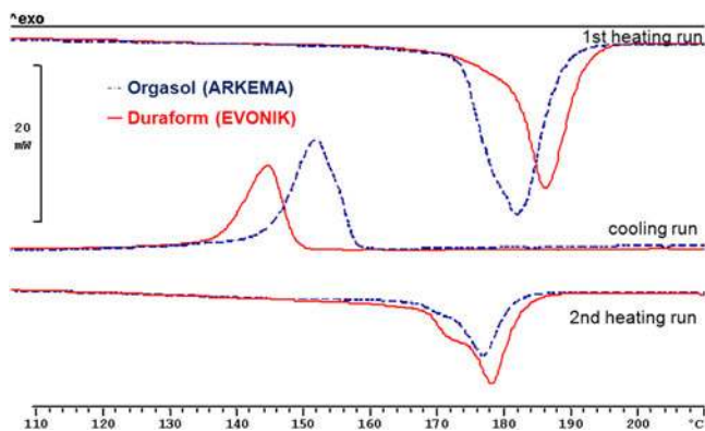
FIG. 7. Comparison of two SLS polyamide 12 (Duraform PA and Orgasol).
