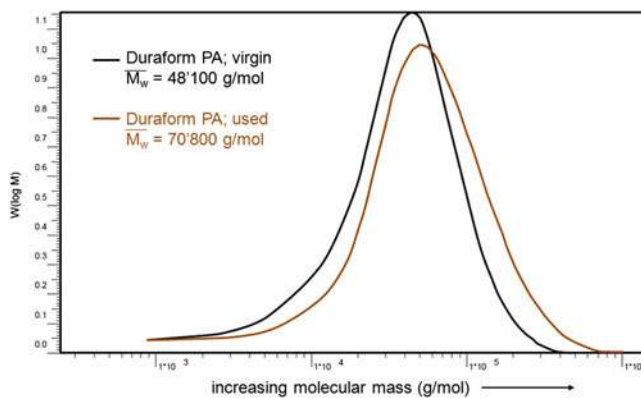
FIG. 11. Comparison of weight average molecular mass from virgin and aged polyamide 12.
