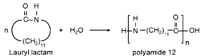
FIG. 9. Synthesis of polyamide 12 from lauryl lactam.
