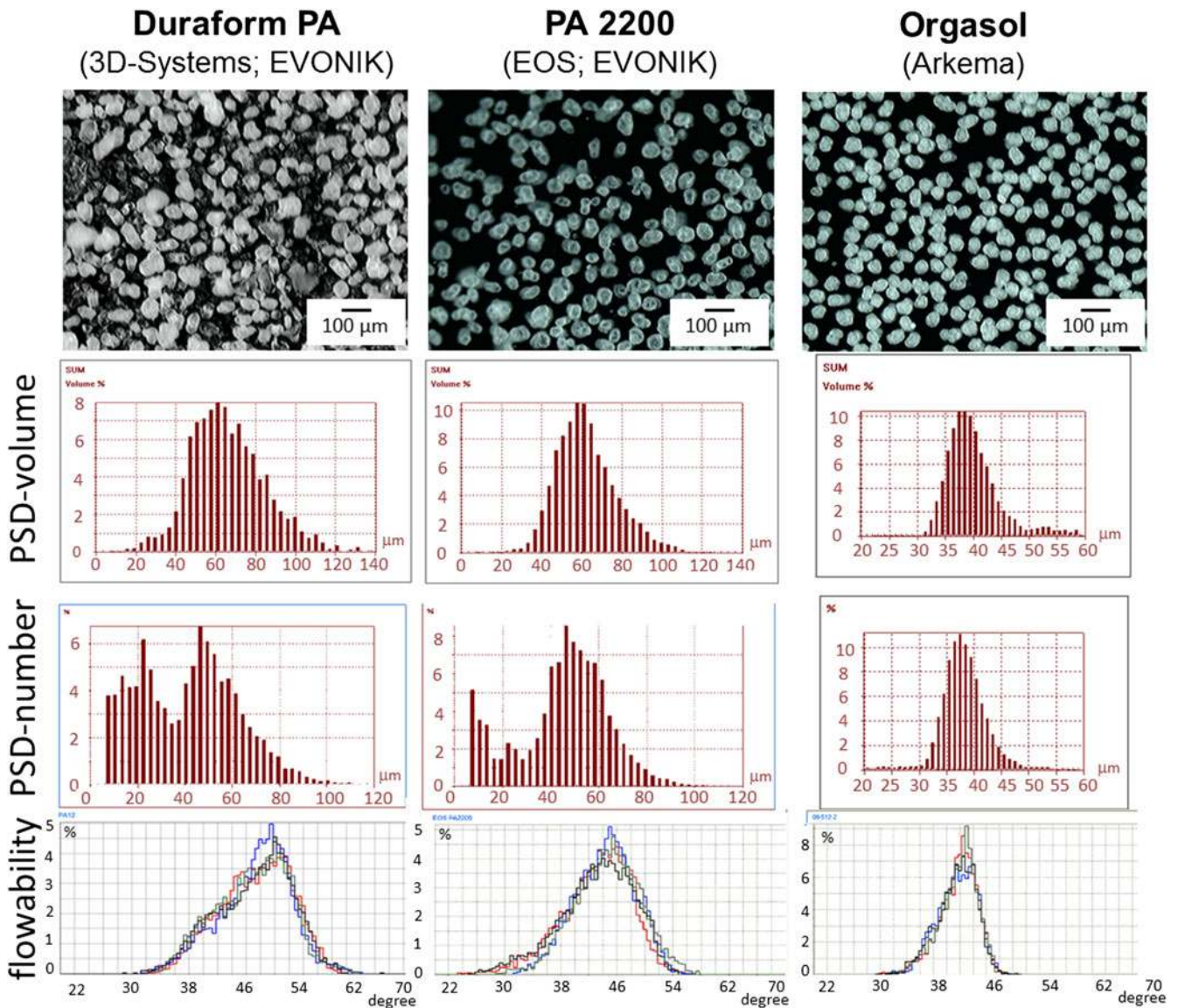
FIG. 8. Distribution of commercial SLS powders regarding particle size and flowability.
