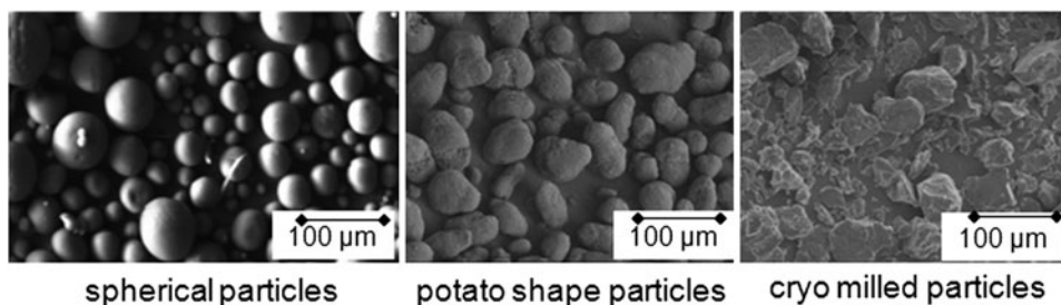
FIG. 3. Particle shapes attainable by different production technologies.
