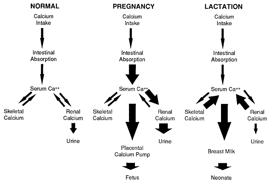
FIG. 5. Schematic illustration contrasting the adaptive processes of calcium homeostasis in human pregnancy and lactation, as compared with normal. The thickness of arrows indicates a relative increase or decrease with respect to the normal, nonpregnant state.
