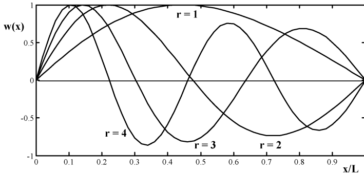
Fig.1: Mode shapes for beam with linearly variable depth ( \alpha = 0.2 , n = 1 , \lambda = 10 )
