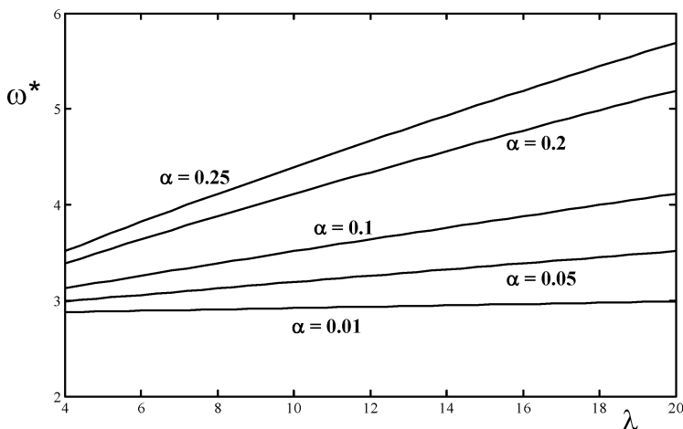
Fig.4: Variation of fundamental natural frequency with slenderness ratio \lambda ( n = 1, r = 1 )
