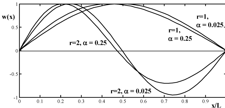
Fig.2: Effect of nonlinearity factor \alpha on mode shapes ( r = 1, 2 , n = 1 , \lambda = 10 )
