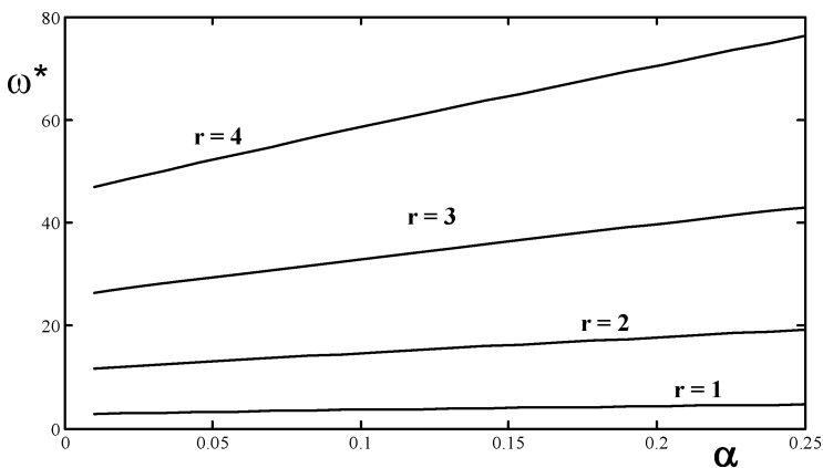
Fig.3: Variation of the First Four Eigen Values with \alpha ( n = 1, \lambda = 12 )
