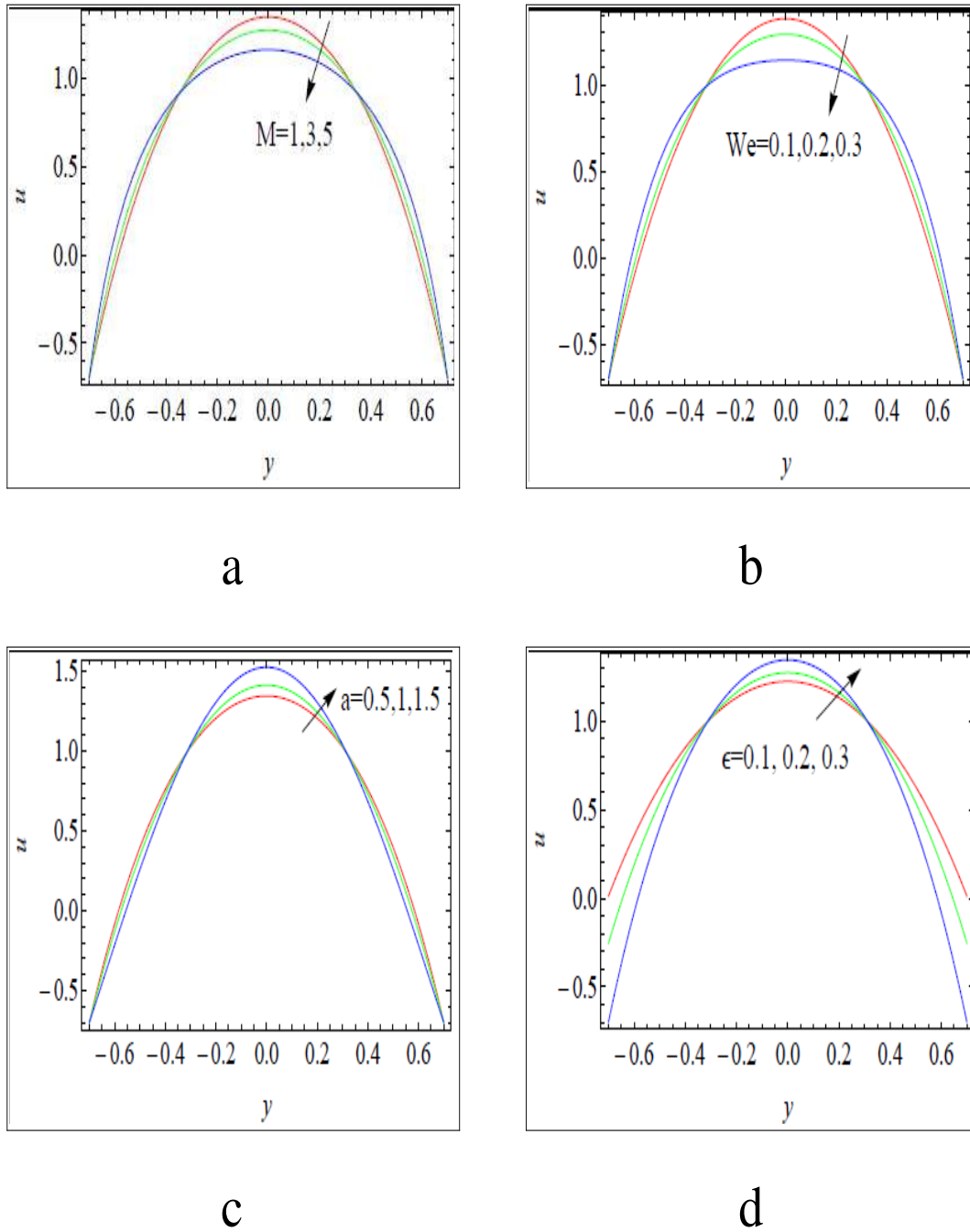
Fig. 3: Axial velocity distributions across channel span with variation in (a) Hartmann number ( M ), (b) Weissenberg number ( We ), (c) Slip parameter ( a ), (d) Cilia length ( \epsilon ), for \alpha=0.4 , \beta=0.4 , \mu=1 , \eta=1 , Q^{\text{cilia}}=1.5 .
