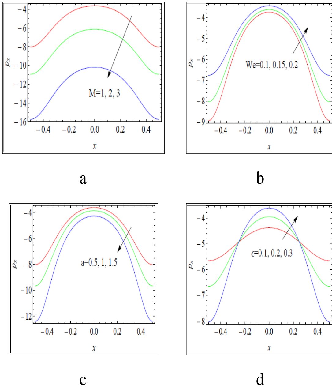
Fig. 2: Axial pressure distributions with variation in (a) Hartmann number ( M ), (b) Weissenberg number ( We ), (c) Slip parameter ( a ), (d) Cilia length ( \epsilon ), for \alpha=0.4 , \beta=0.4 , \mu=1 , \eta=1 , Q^* = 1.5 .
