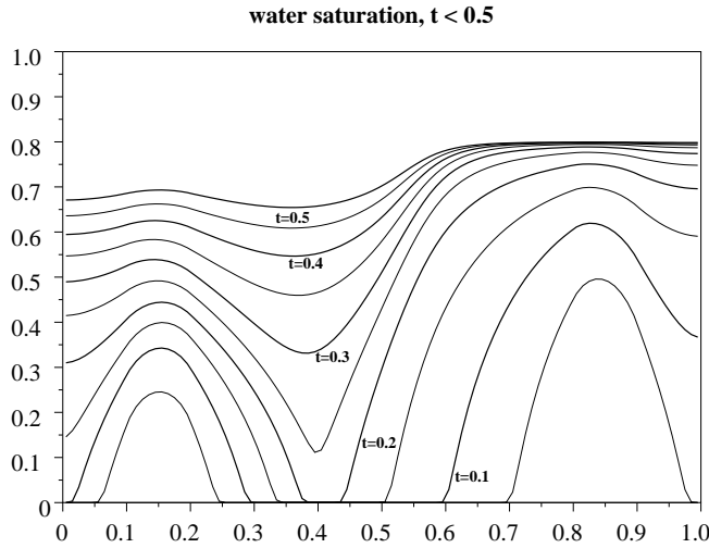
FIGURE 3. Water saturation evolution from t = 0 to t = 0.5 . |u_w| := mean value, and u_w(\text{prod}) := value at the production well.
