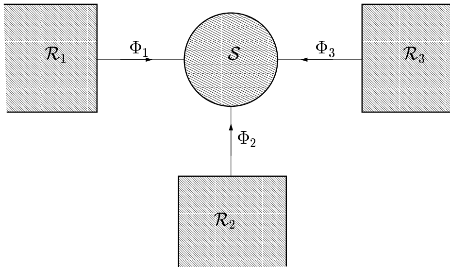
Figure 2: The energy currents \Phi_k .
