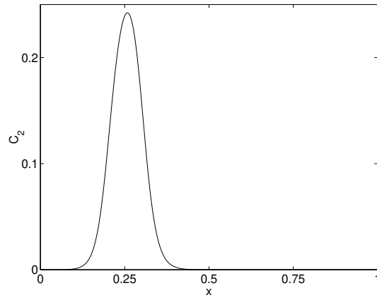
Fig. 11. The function C_2(x) in Example 1.
