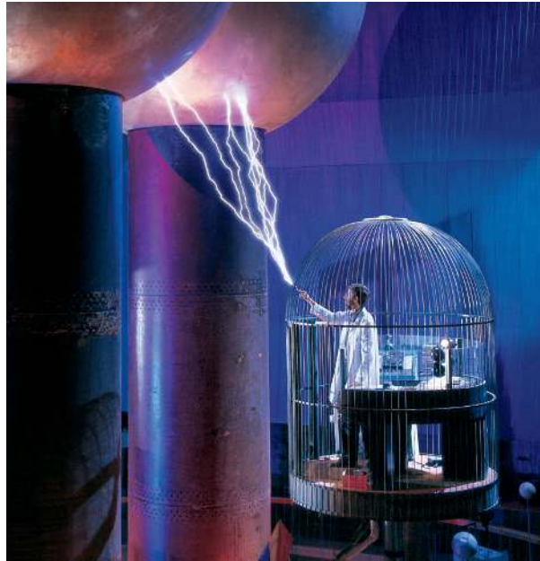
Fig. 1.1 Dramatization of the Faraday cage effect. This image shows the giant Van de Graaff generator at the Museum of Science in Boston. (Photo © Steve Marsel, courtesy of the Museum of Science, Boston.)
