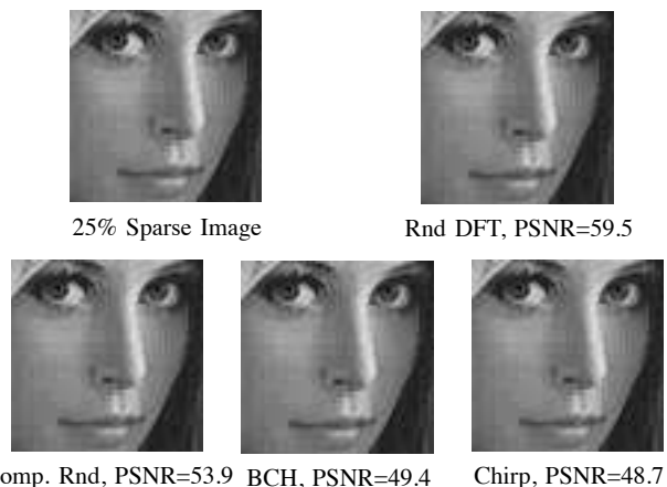
Fig. 9. Comparison of utilizing different sampling matrices in order to compress a 65 \times 65 Lena image with sparsity of 25%. All the employed matrices are 2400 \times 4225 ; from the 7-ary 2400 \times 117649 BCH-based matrix which has the coherence \frac{1}{48} , we have kept only the first 4225 columns.
