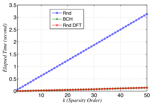
Fig. 8. Comparison of the required time for retrieving sparse 15625 \times 1 signals utilizing a 5-ary BCH-based matrix, complex-valued random matrices and random sub-matrices of the DFT matrix all of size 624 \times 15625 vs. sparsity order of the source signal.
