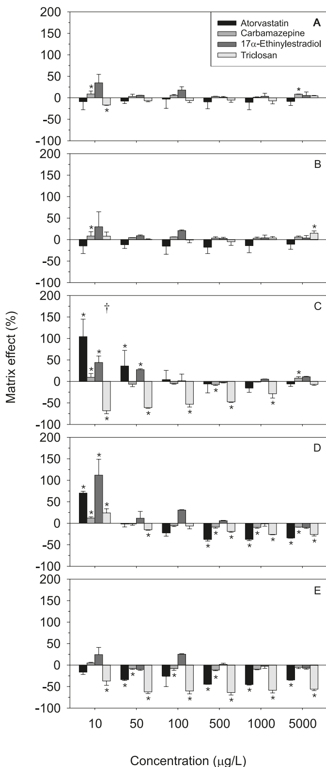
Fig. 1. Matrix effects (mean \pm SEM; n = 2 ) in two types of reconstituted water (A, B), sediment extracts (C), and biota extracts (D, Chironomus tentans ; E, Hyalella azteca ) with increasing standard concentration on four pharmaceuticals and personal care products. The matrix effect signifies the compound is X\% more or less recoverable than in the absence of the matrix of interest. * denotes values significantly different from zero ( p < 0.05 ). † denotes concentrations below the limit of detection (LOD) and should be interpreted with caution.
