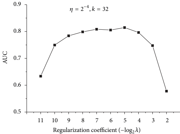
FIGURE 5: The AUC results of models based on different penalization coefficients. Learning rate remains the same. The dimension of feature vectors is set as 32.
