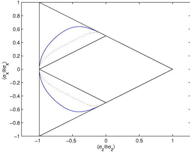
FIG. 1. (Color online) Convex sets of the possible reduced density operators of translational invariant states in the XX - ZZ plane: the big triangle represents all positive density operators, the inner parallelogram represents the separable states, the union of the separable cone and the convex hull of the full curved line is the complete convex set in the case of a 1D geometry, and the dashed lines represent extreme points in the 2D case of a square lattice. The singlet corresponds to the point with coordinates (-1, -1) .
