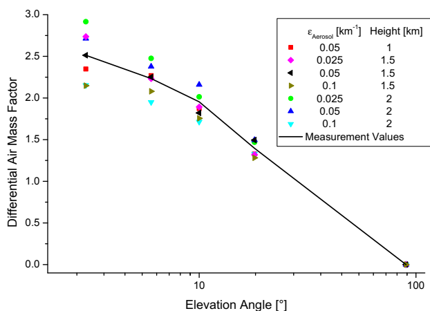
Fig. 3. From measurements calculated O_4 DAMFS (black line) compared with modeled O_4 DAMF for different homogeneously mixed aerosol layers (see legend) as a function of the logarithm of the elevation angle for an SZA of about 40^\circ at MIT.
