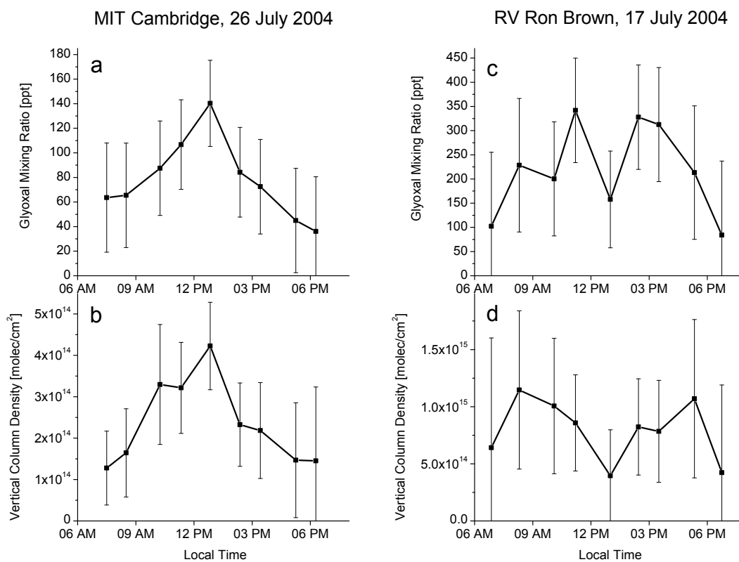
Fig. 5. CHOCHO mixing ratios and VCDs at MIT in Cambridge on 26 July 2004 (a and b) and RV Ron Brown on 17 July 2004 (c and d) retrieved by radiative transfer modeling from CHOCHO DSCDs.
