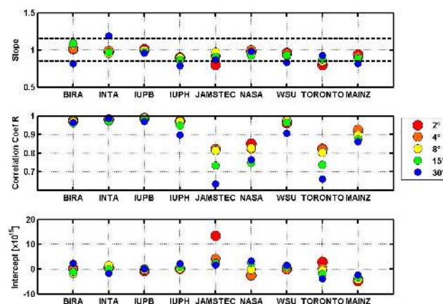
Fig. 7. Straight-line slopes, correlation coefficients and intercepts of HCHO slant columns against those of the reference, for each instrument and all off-axis elevation angles. The dotted lines in the first panel correspond to values of 1.15 and 0.85.
