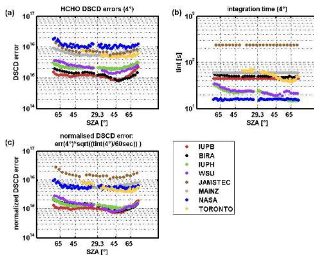
Fig. 17. Comparison of HCHO DSCD errors (molec \text{cm}^{-2} ) retrieved by each participating group for the case of 4^\circ elevation, based on measurements from 4 July 2009. (a) DSCD errors from DOAS evaluations, (b) corresponding integration times, (c) DSCD errors normalized by their integration exposure times.
