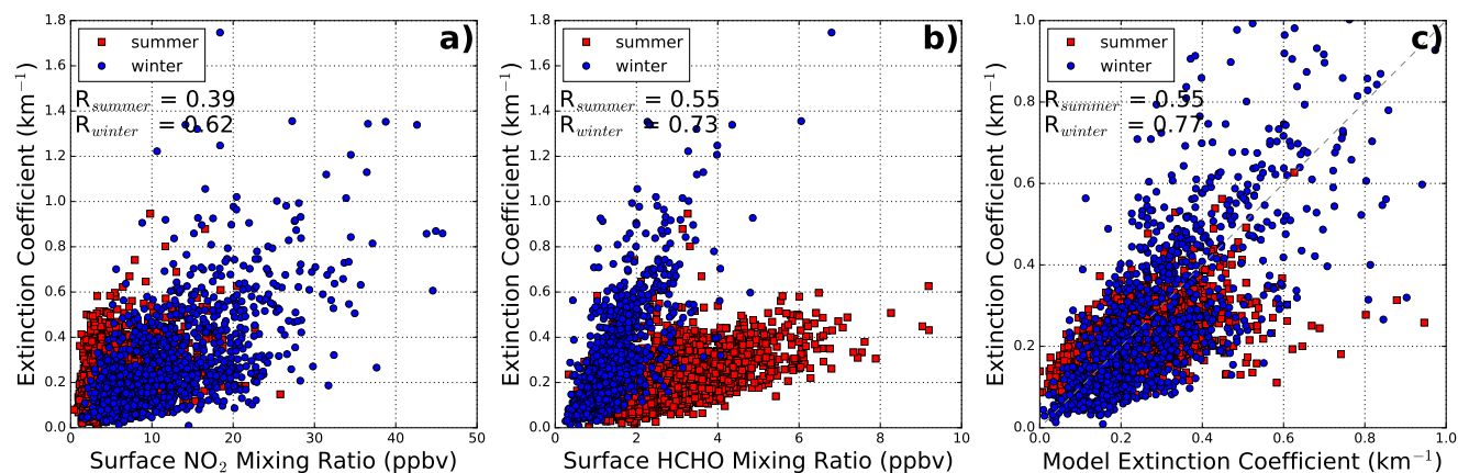
Figure 6. (a) shows the correlation between surface aerosol extinction coefficients ( \varepsilon_{\text{surf}} ) and \text{NO}_2 mixing ratios. (b) shows the correlation between \varepsilon_{\text{surf}} and HCHO mixing ratios. (c) shows the scatter plot of measured and modeled surface aerosol extinction coefficients. Data measured in summer (June, July and August, red markers) and winter (December, January and February, blue markers) are shown.
