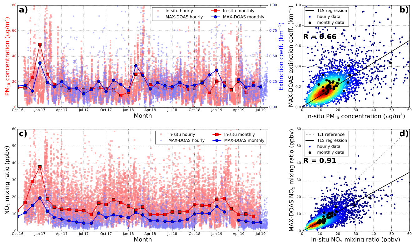
Figure 7. (a) Time series of surface aerosol optical extinction coefficients \varepsilon_{\text{surf}} at 360 nm retrieved from MAX-DOAS observations (blue curve) and \text{PM}_{10} concentrations measured by the air quality monitoring station (red curve). (b) Scatter plot of \varepsilon_{\text{surf}} against \text{PM}_{10} concentrations. (c) Time series of surface \text{NO}_2 mixing ratios measured by the MAX-DOAS (blue curve) and the air quality monitoring station (red curve). (d) Scatter plot of the \text{NO}_2 mixing ratios measured by the MAX-DOAS against the air quality monitoring station measurements. Correlation coefficient and total least squares regression lines are calculated based on monthly averaged data.
