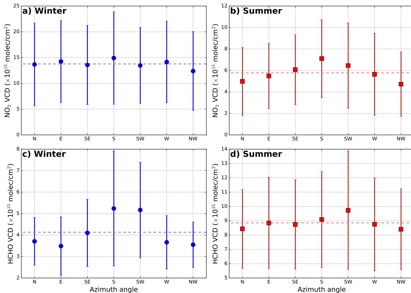
Figure 4. MAX-DOAS measurements of NO 2 VCD for different viewing azimuth angles for (a) winter (December, January and February) and (b) summer (June, July and August). HCHO VCDs measured in winter and summer are shown in (c) and (d), respectively. Error bars indicate the 1 \sigma standard deviation variation range. Note that the scale of y-axis of each subplot is different.
