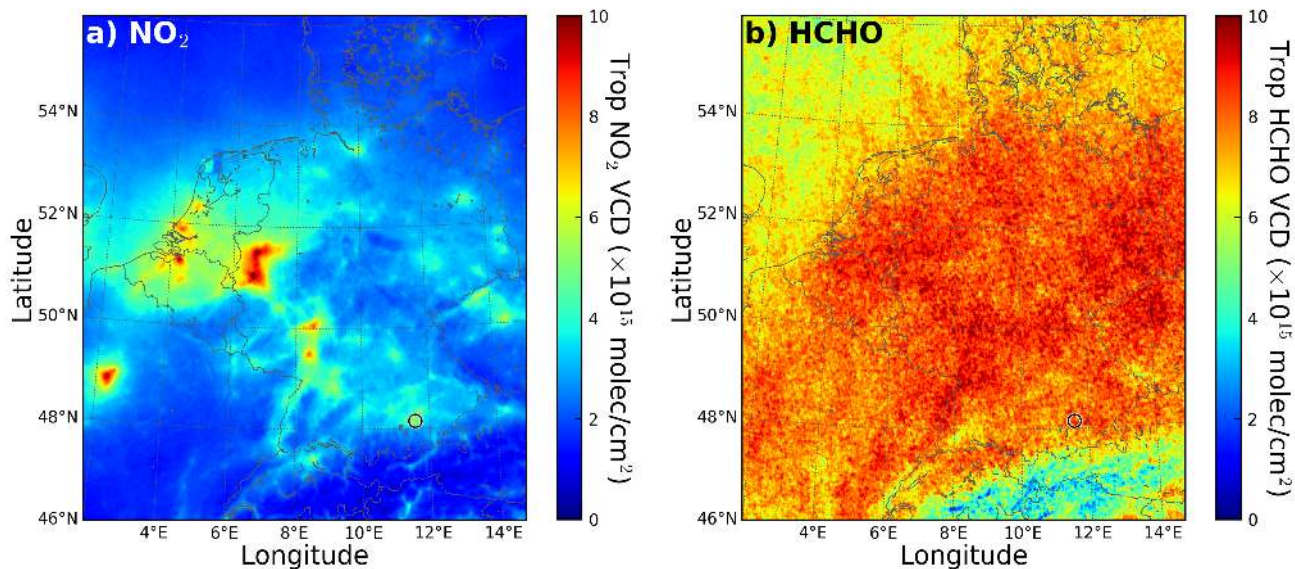
Figure 3. Annual average TROPOMI tropospheric (a) \text{NO}_2 and (b) HCHO VCDs over Germany and its surrounding regions. The circle marker indicates the location of Munich. Data from May 2018 to April 2019 are used in the calculation of average maps. Values above or below the range of the color scale are set to the maximum or minimum value of the color scale.
