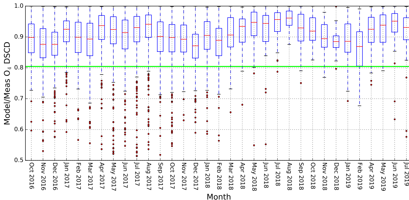
Figure A1. Monthly statistic of measured O 4 DSCD exceeding pure Rayleigh simulation. The ratios between modeled and measured O 4 DSCDs for observations taken with elevation angle of 15° are shown. The green line indicates the 10 th percentile (0.804).
