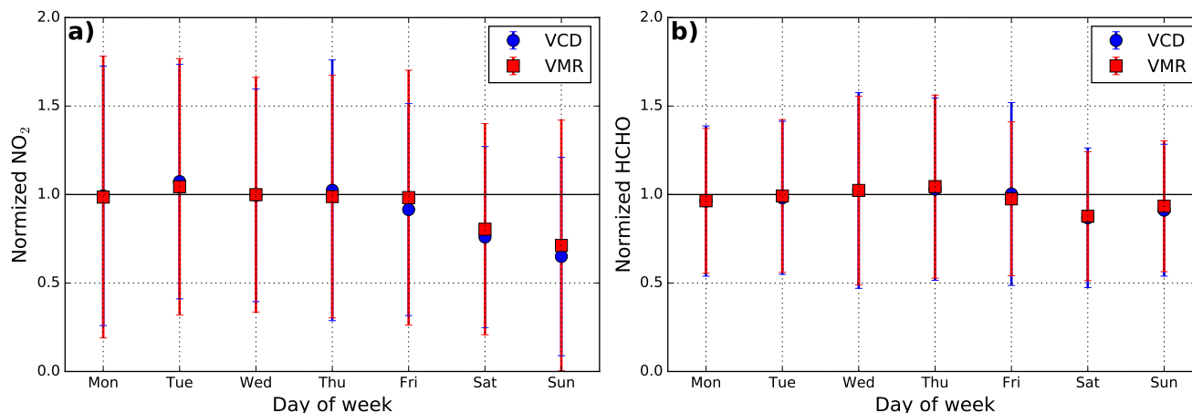
Figure 5. Average weekly cycle of (a) NO 2 and (b) HCHO measured by the MAX-DOAS instrument. Data are normalized by dividing by the mean weekday value (Monday to Friday). Both vertical column (blue circle) and surface mixing ratio (red square) are shown. Error bars indicate the 1 \sigma standard deviation variation range.
