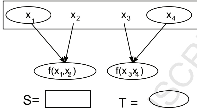
Figure 11: Graph G_\Gamma for the butterfly network.
