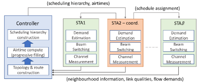
Fig. 3: High-level overview of the envisioned system. WiHAUL runs on the controller and computes flow airtime allocations and schedules, based on topology information and paths computed by routing logic. Scheduling hierarchy and airtimes sent to a scheduling coordinator, which dictates the TX/RX timing to backhaul nodes.
