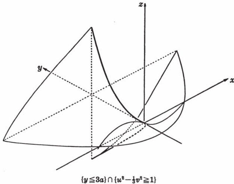
(y \leq 3a) \cap \{u^2 - \frac{1}{3}v^2 \geq 1\} FIGURE 3. Conjugate of Enneper's surface of 2nd kind.
