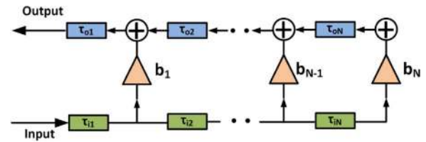
Fig. 1. General diagram of a transversal filter.
