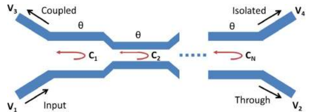
Fig. 7. N -section directional coupler.
