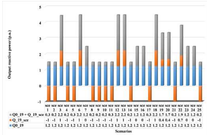
Fig. 7. Output reactive power of generating unit 19 in first and second level of optimization
