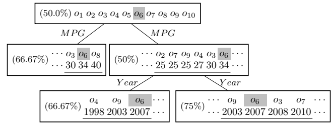
Fig. 4. Diversified predicates selected by DBA
