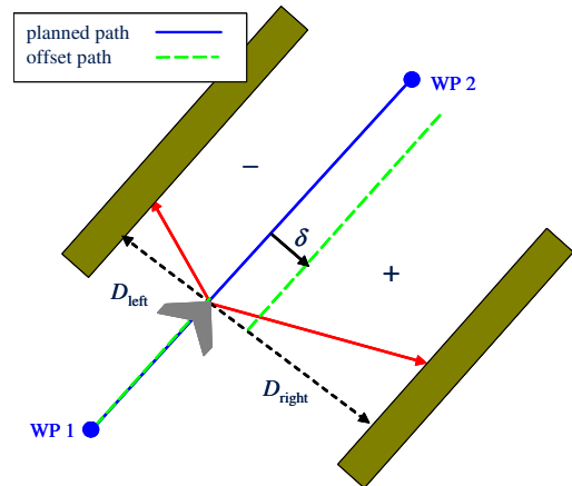
Fig. 12. Using the measurements from the optic flow sensors, the planned path (solid blue) is shifted by \delta to create a new desired path (dashed green) that is centered between the canyon walls.
