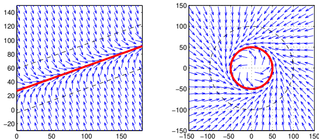
Fig. 6. Path following in wind is accomplished by creating a vector field of desired course commands based on the lateral deviation from the path. The figure on the left shows a possible vector field for a straight-line waypoint path segment. The figure on the right shows a possible vector field for orbit following.
