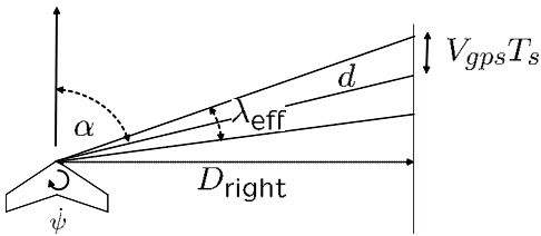
Fig. 4. The optic flow sensor is used to compute the distance to an obstacle based on the distance traveled between samples ( V_{\text{gps}} T_s ) and the effective field of view \lambda .
