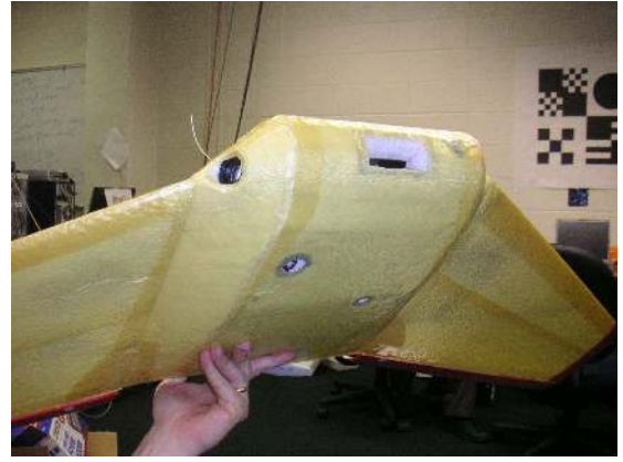
Fig. 2. Sensors used for collision avoidance. The round hole on the right and the large hole on the belly are the optic flow sensors. The square hole in the center is the laser ranger, and the other two round holes are for electro-optical cameras.
