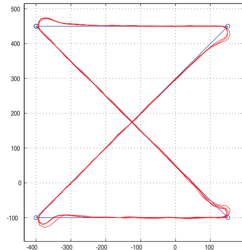
Fig. 7. This figure shows telemetry data for four consecutive traversals of a waypoint path. Wind speeds during the flight were 20% of the MAV airspeed. Note the repeatability of the trajectories even in significant wind.
