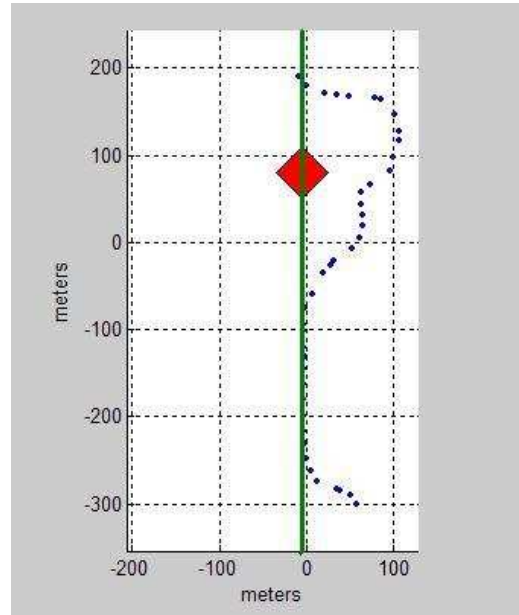
Fig. 10. Flight results for collision avoidance using a laser ranger. The green line indicates the planned waypoint path, and the dotted line indicates the GPS track of the MAV.
