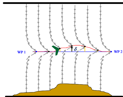
Fig. 13. The adjusted path (red) is offset from the preplanned path (blue) by the calculated offset ( \delta ) at each time step to center the desired path between the canyon walls, thus shifting the vector field along with it.
