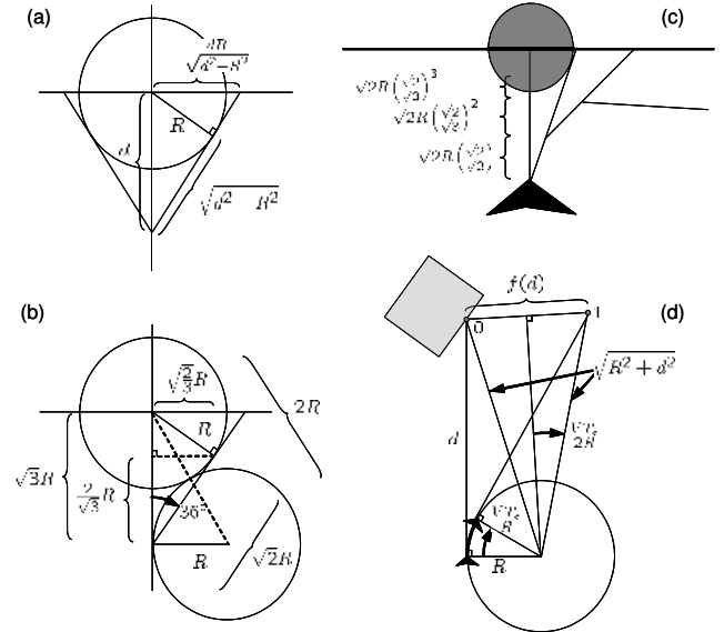
Fig. 9. (a) The waypoint path is constructed so that it is perpendicular to the map obstacle. The radius R ensures collision free passage around the map obstacle. (b) The maximum heading change in waypoint paths is when the MAV must make a full bank to maneuver around the obstacle. (c) An approximation of the minimum distance required to avoid a straight wall if the laser is only sampled when the MAV is on the waypoint path. (d) the geometry used to calculate the distance between two consecutive laser updates.
