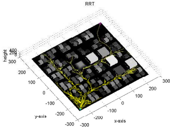
Fig. 5. This figure shows the growth of an RRT path tree through a simulated urban environment. The algorithm is terminated once a feasible path to the destination (red X) is found.
