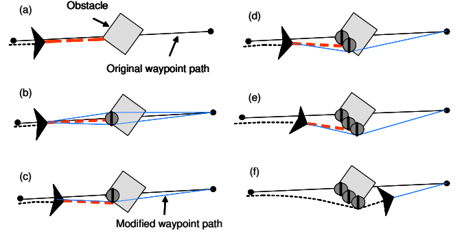
Fig. 8. Obstacle avoidance algorithm. (a) The laser detects the obstacle. (b) A map obstacle of radius R is inserted into the map, and two candidate waypoint paths are constructed. (c) A modified waypoint path is randomly selected. (d) The obstacle is again detected by the laser and another map obstacle is constructed. (e-f) The process repeats until the MAV is able to maneuver around the obstacle.
