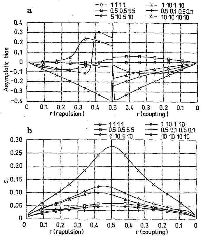
Fig. 8a, b a Asymptotic bias of the classical MLE (using Newton-Raphson iterations) of the recombination fraction, r , between two markers affected by a zygotic selection. b Asymptotic standard error of the MLE (equation A.6; see Appendix) in the same conditions, for an F_2 population of 100 individuals. The numbers in the legends denote the values of u_1, u_2, v_1 and v_2 , respectively
