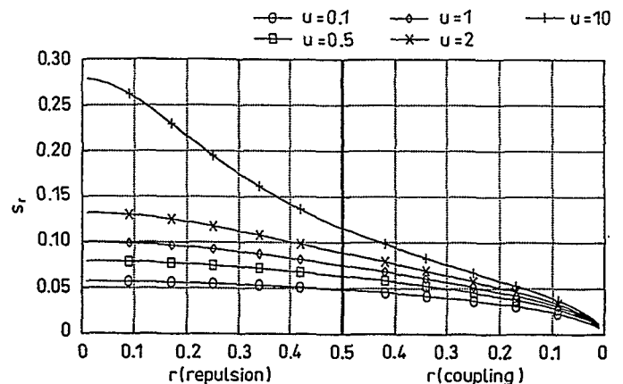
Fig. 1 Asymptotic standard error of the classical estimate of the recombination fraction, r , between two dominant markers, one being affected by a zygotic selection with intensity u ( F_2 population of 100 individuals)
