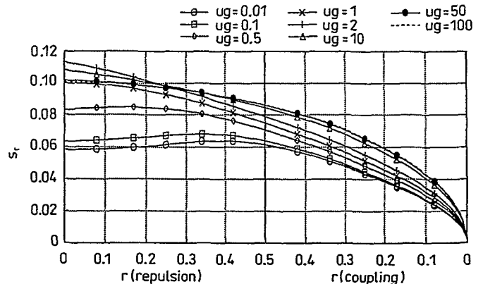
Fig. 6 Asymptotic standard error of the fully efficient estimate of the recombination fraction, r , between two dominant markers, one being affected by a gametic selection with intensity u_g ( F_2 population of 100 individuals)
