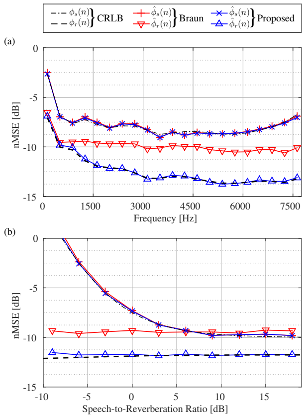
Fig. 2. Normalized MSE of PSD estimation of the proposed PSD estimators (Proposed) and the PSD estimators from [17] (Braun) as a function of: (a) frequency (SRR: 0 dB), (b) SRR (frequency: 1500 Hz). M = 4 , L = 10 .
