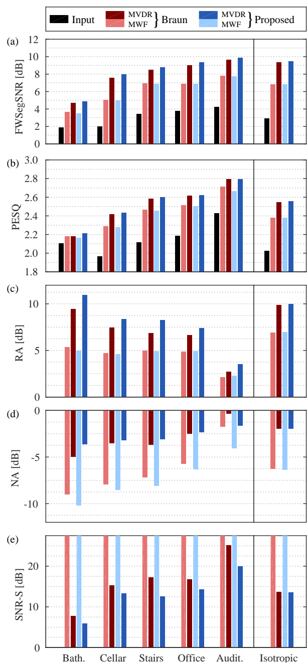
Fig. 3. (a) FWSegSNR, (b) PESQ, (c) RA, (d) NA, and (e) SNR-S scores obtained by using MWFs and MVDR beamformers based on the PSD estimators from [17] (denoted “Braun”) and the proposed estimators (denoted “Proposed”). Scores obtained from the unprocessed input signal (“Input”) are also included.
