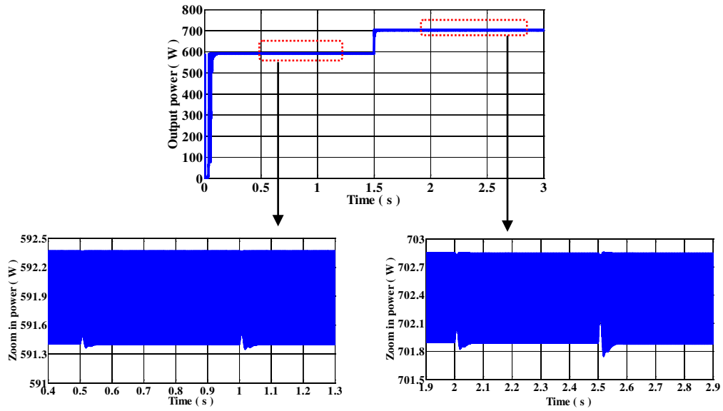
Figure 15. Influence of the load behavior on power.
