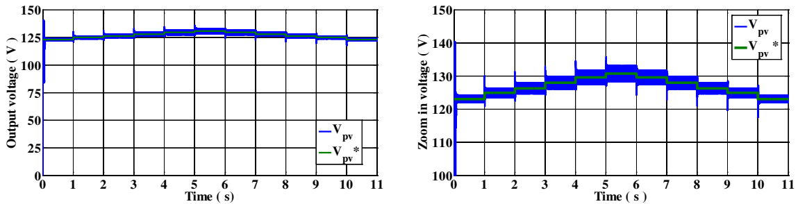
Figure 11. The output voltage of PV array based on MPPT control.
