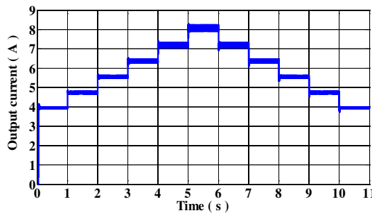
Figure 12. The output current of PV array based on MPPT control.
