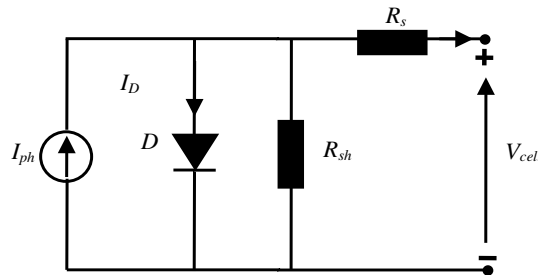
Figure 2. Equivalent circuit of a photovoltaic cell.
