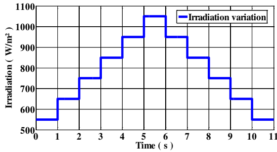
Figure 9. Irradiation profile.
