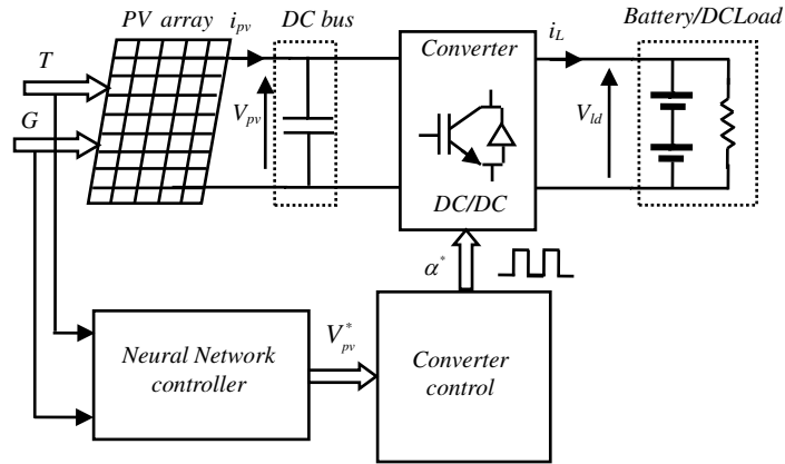
Figure 1. System configuration.
