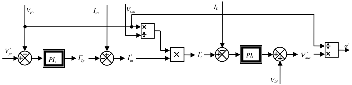
Figure 5. Structure of the proposed power stage control.
