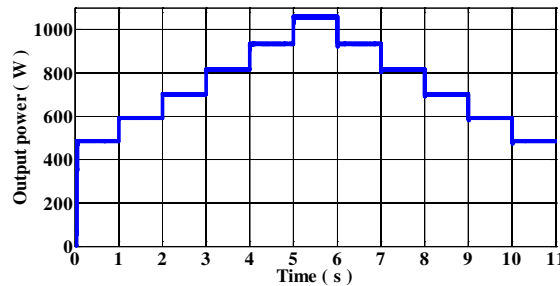
Figure 10. The output power of PV array based on MPPT control.
