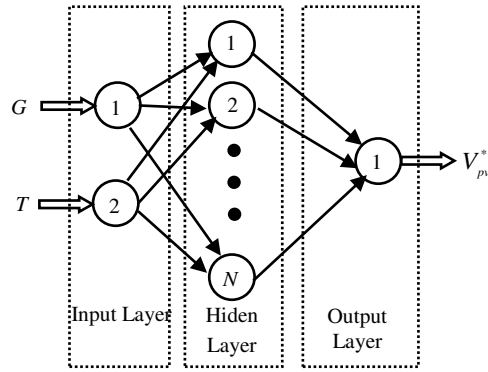
Figure 4. The neural network architecture.
