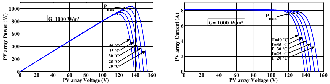
Figure 7. Simulated P-V and I-V characteristics of the PV array at constant solar radiation.
