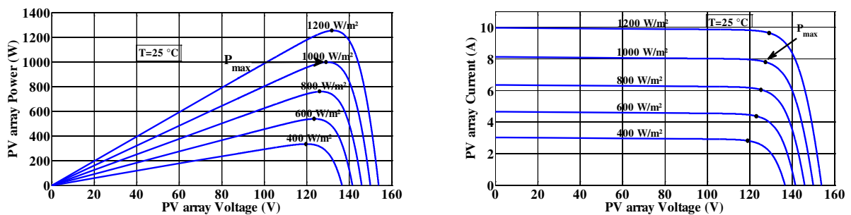
Figure 6. Simulated P-V and I-V characteristics of the PV array at constant temperature.
