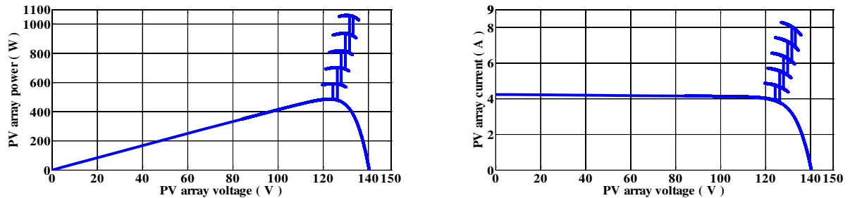
Figure 13. P-V and I-V characteristics with the proposed MPPT control method under irradiation changes.
