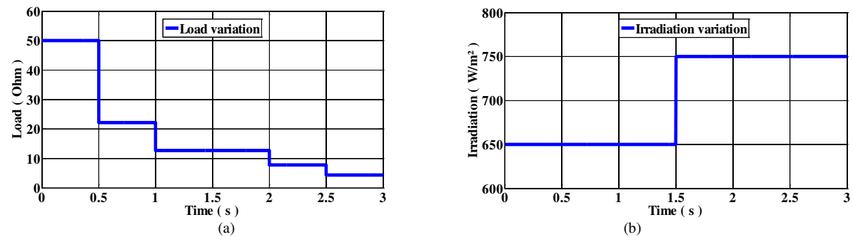
Figure 14. (a) Simulation of the resistive load variation according to time; (b) Irradiation profile.
