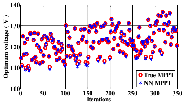
Figure 8. The neural network response and the corresponding targets for the test set.
