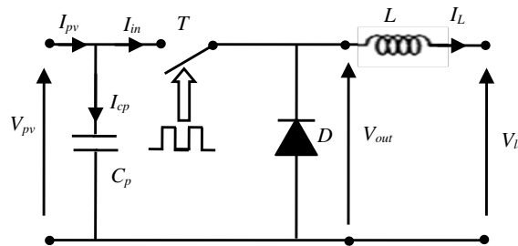
Figure 3. Equivalent circuit of the buck converter.
