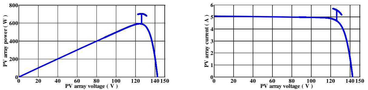
Figure 18. P-V and I-V characteristics with the proposed MPPT control method under load and irradiation variations.
