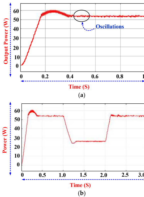
Figure 14. Output power from PSO for (a) 1000\text{W}/\text{m}^2 ; (b) irradiance is varied from 1000\text{W}/\text{m}^2 to 500\text{W}/\text{m}^2 at 1 s then increased to 1000\text{W}/\text{m}^2 at 2 s.
