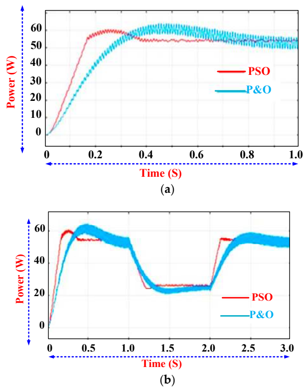
Figure 15. Comparison of output power from PSO based MPPT and P&O based MPPT for (a) 1000\text{W}/\text{m}^2 ; (b) irradiance is varied from 1000\text{W}/\text{m}^2 to 500\text{W}/\text{m}^2 .
