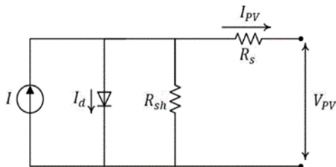
Figure. 2 Photovoltaic cell model
