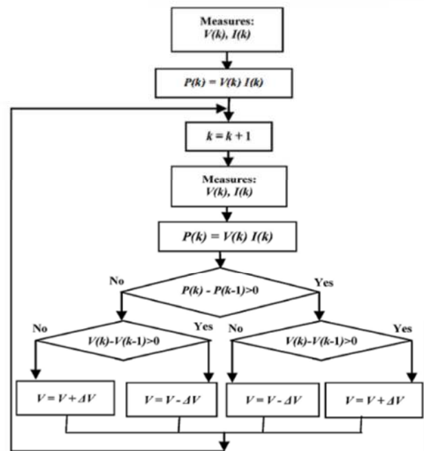
Figure 5. Flowchart for conventional Perturb and Observe algorithm.
