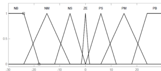
Fig. 6 Membership Functions of the 1 st Input Variable 1 st ( \Delta P_{pv} )
