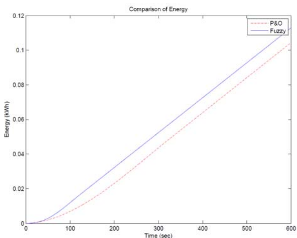
Fig. 13 Energy obtained from the both controllers.
