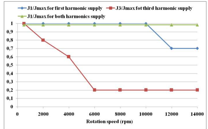
Fig. 9. Current supply for each control strategy ( J_{\max}=10\text{ A/mm}^2 )
