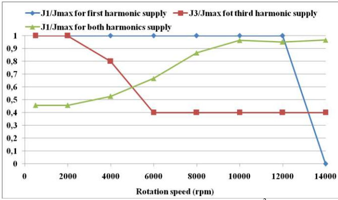
fig. 6. Current supply for each control strategy ( J_{\max}=5\text{ A/mm}^2 )
