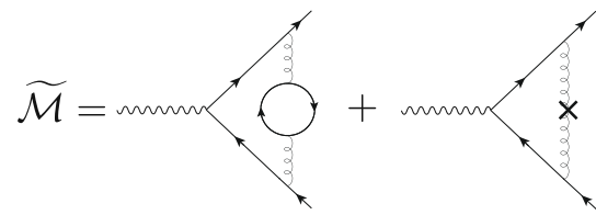
Fig. 7 Diagrams entering in the UV renormalisation of scattering process \gamma^* \rightarrow b\bar{b}
