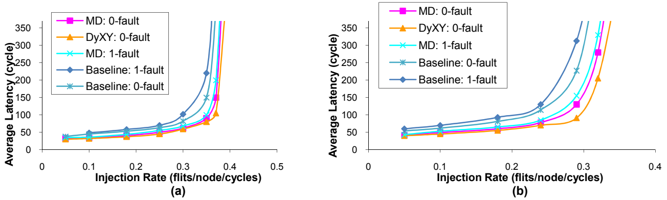
Fig. 8. Performance analysis of MD and the baseline method in 4x4 mesh network (a) under uniform traffic profile (b) hotspot traffic profile in fault-free, 1-faulty link cases.
