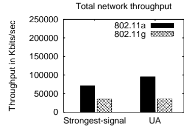
Figure 4: Comparison between UA in isolation, and strongest-signal affiliation, for both 802.11a and 802.11g.
