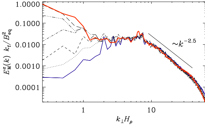
Fig. 18. Normalized spectra of B_z from DNS Run a30/4 at normalized times t_{t0}/H_p^2 \approx 0.2, 0.5, 1, 2, 5, 10, and 20 , for \hat{g} \equiv g/c_s^2 k_f = 4 .
