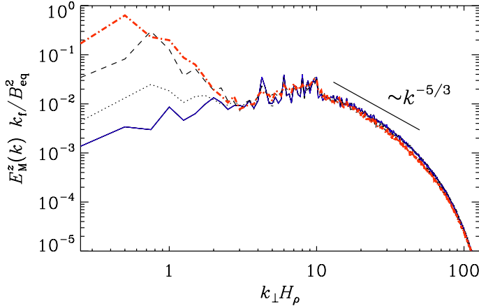
Fig. 19. Normalized spectra of B_z from DNS Run A40/1 at normalized times t_{t0}/H_p^2 \approx 0.2, 0.5, 1, and 2.7 with k_f H_p = 10 and k_1 H_p = 0.25 .
