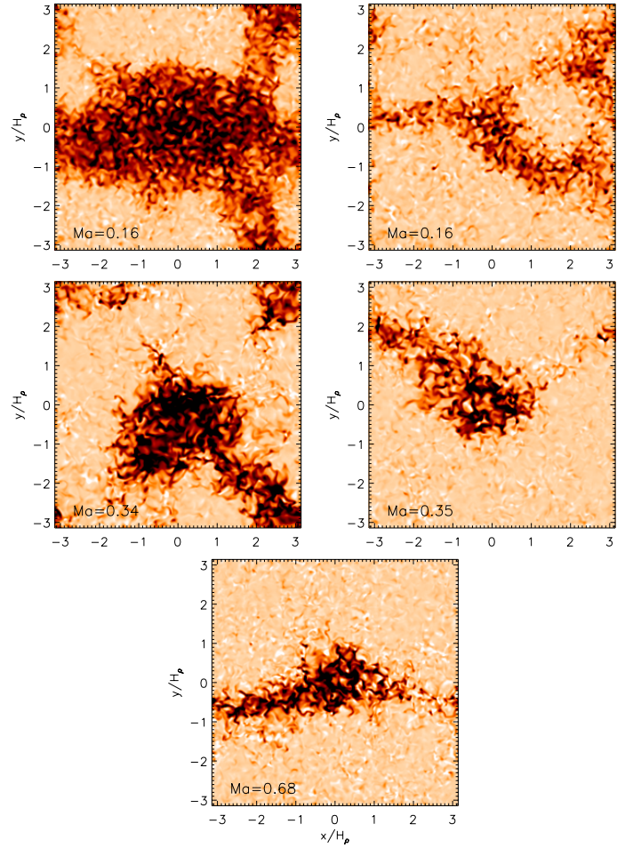
Fig. 22. Surface appearance of the vertical magnetic field, B_z^{\max} , in the ILES simulations with different Mach numbers ( top to bottom ). The color coding shows B_z^{\max} / B_{eq} in the range of -0.1 (white) to +1.0 (black). Root-mean-square Mach numbers are given by the labels. For the upper two rows with lower Mach number, the left column is for fixed initial mean field, whereas in the right column the initial field is adjusted between the runs, such that the field strength remains constant relative to the kinetic energy in the background turbulence.
