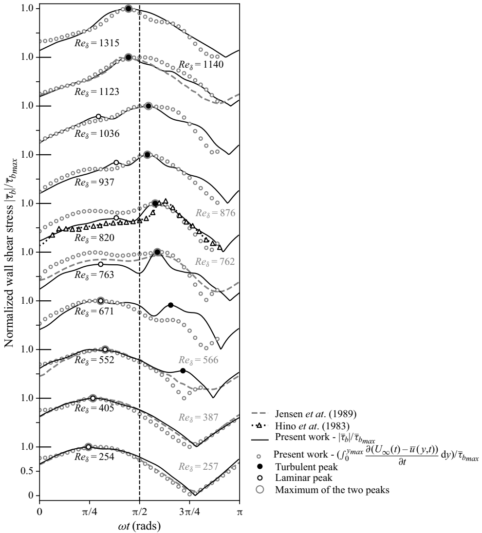
Figure 8. Normalized bed shear stress |\bar{\tau}_b|/\bar{\tau}_{bmax} for various Re_\delta . The peaks associated with the laminar regime are shown with \circ and the peaks associated with the ‘turbulent’/‘transitional’ regime are shown with \bullet . The maximum of the two peaks is shown with \circ (grey). The Re_\delta values for the data by Hino et al. (1983) and Jensen (1989) are shown in grey text.
