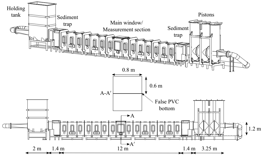
Figure 2. Large Oscillatory Water and Sediment Tunnel (LOWST).
