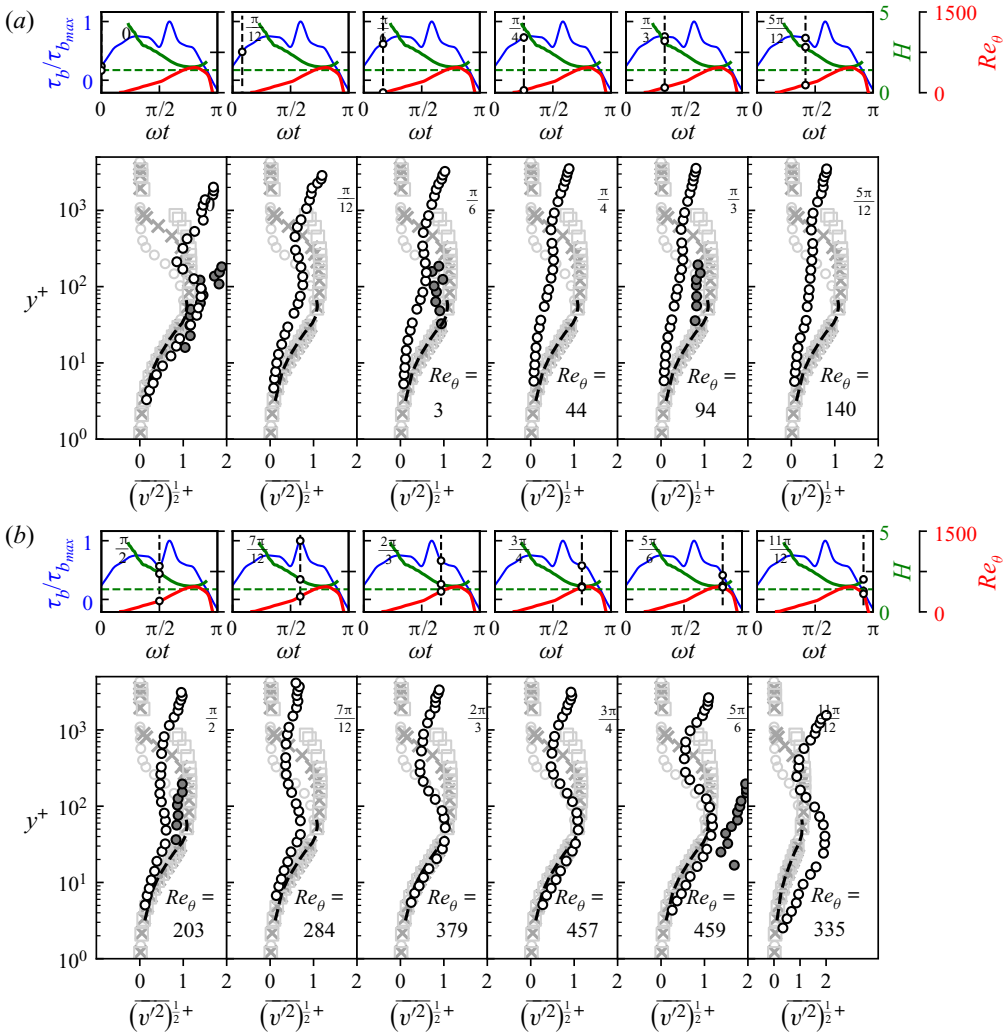
Figure 14. Ensemble-average vertical r.m.s. profiles \sqrt{v^2}^+ for Re_\delta = 763 (the legend is the same as in figure 13).
