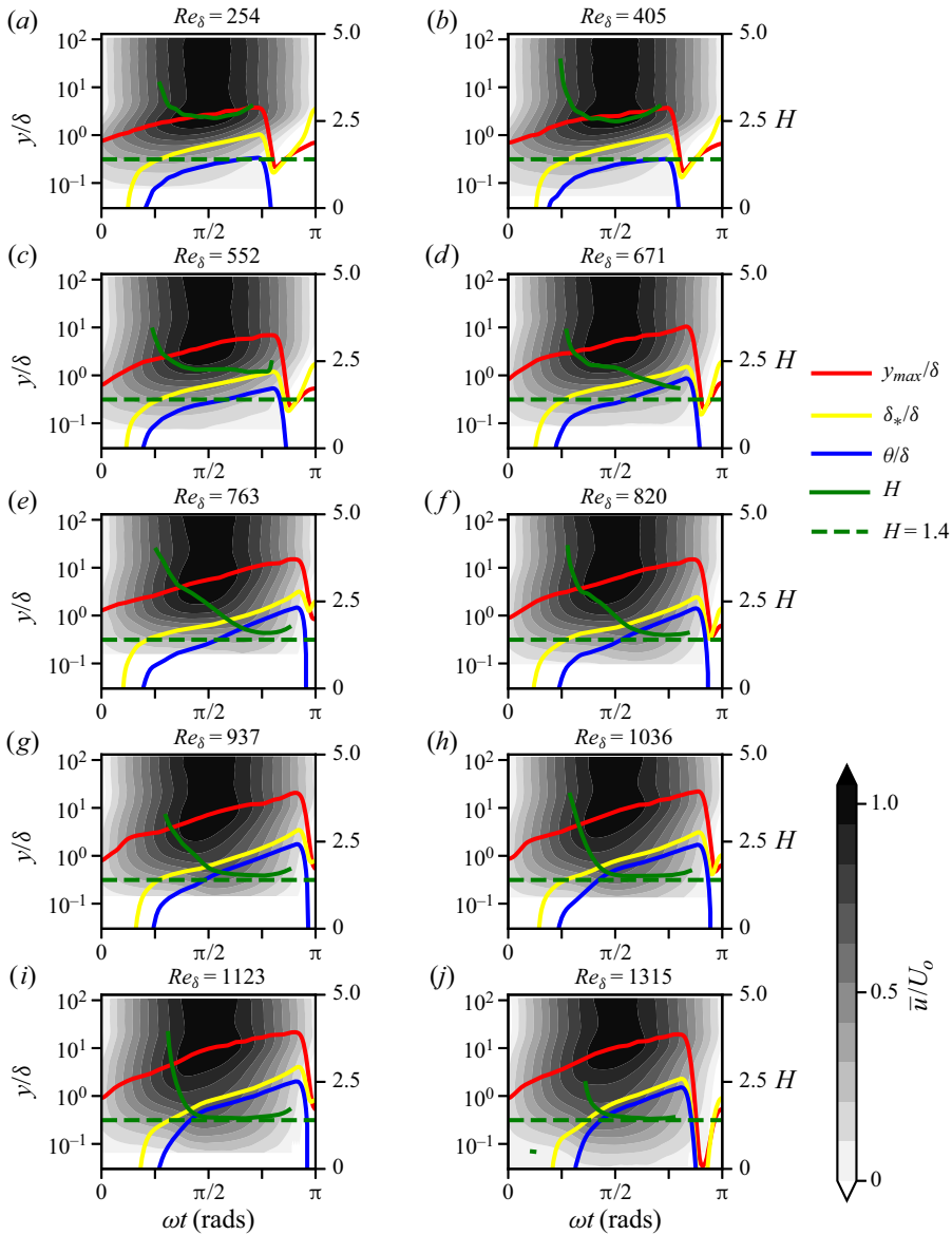
Figure 7. Contour maps of normalized velocity profiles \bar{u}/U_0 . Dimensionless boundary layer thickness y_{max}/\delta , displacement thickness \delta_*/\delta , momentum thickness \theta/\delta and shape factor H . The typical value of H = 1.4 for fully developed unidirectional flow is also shown.
