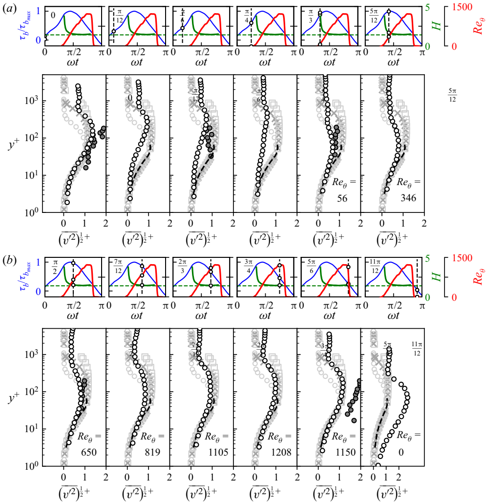
Figure 18. Ensemble-average vertical r.m.s. velocity fluctuation profiles \sqrt{v^2+} for Re_\delta = 1315 (the legend is the same as in figure 17).
