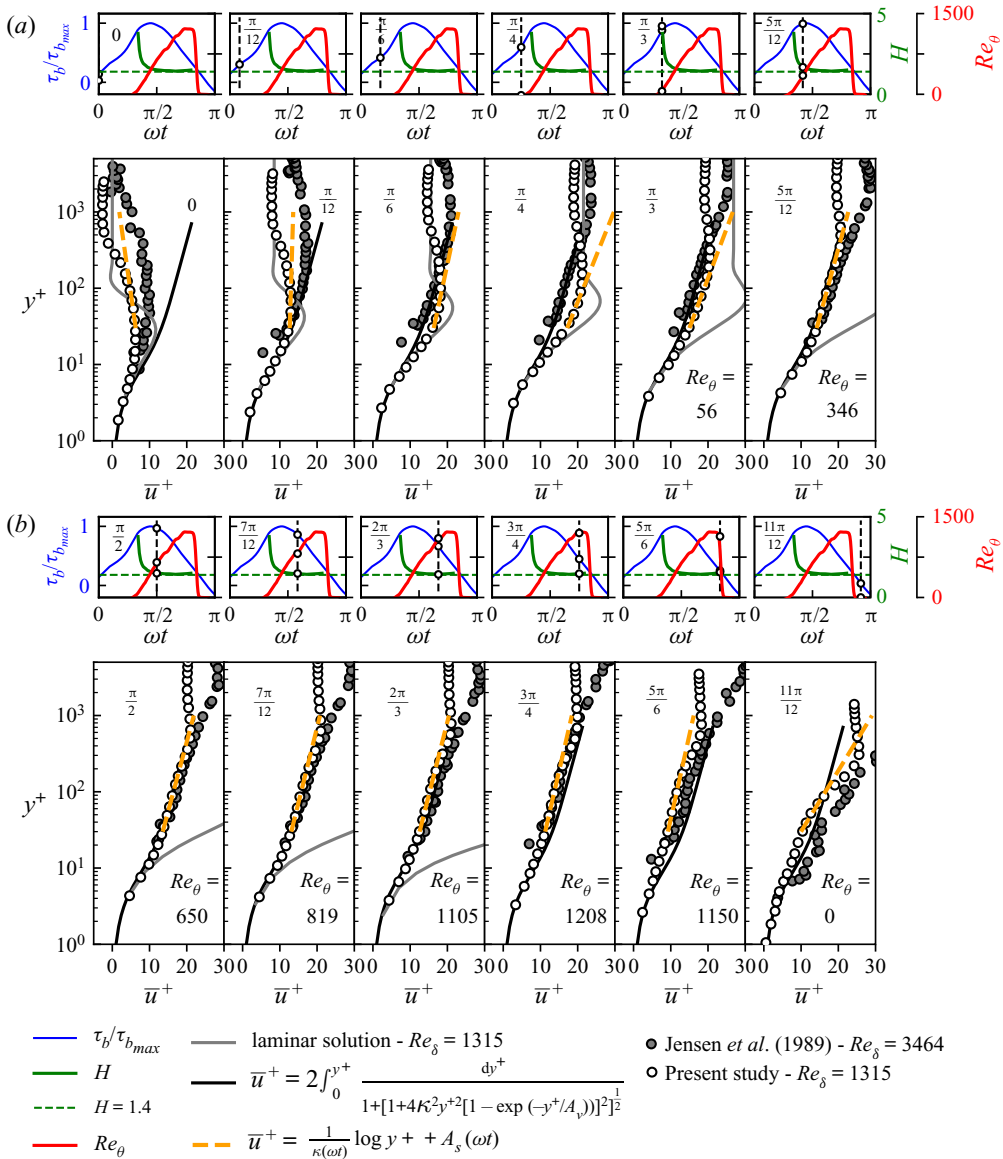
Figure 16. Ensemble-average velocity profiles \bar{u}^+ and logarithmic fit for Re_\delta = 1315 .
