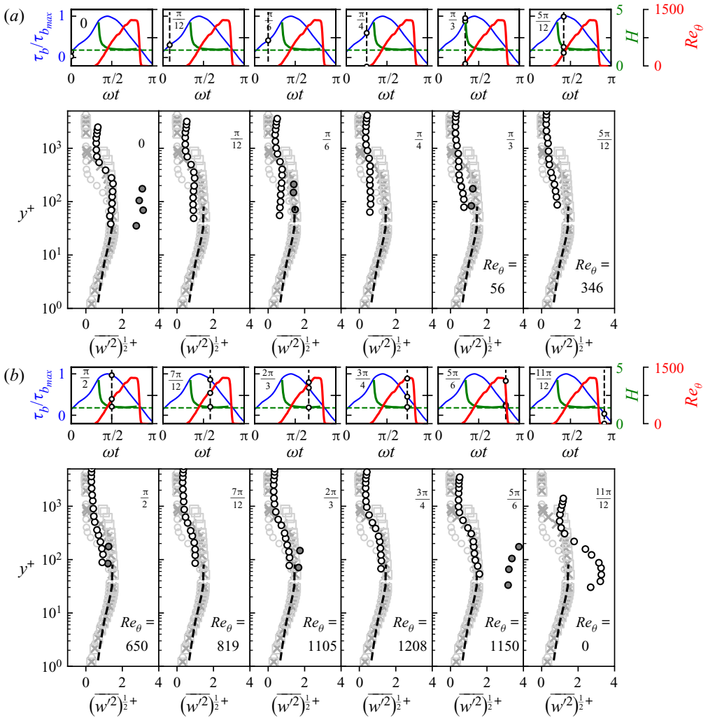
Figure 19. Ensemble-average spanwise r.m.s. velocity fluctuation profiles \sqrt{w'^2} for Re_\delta = 1315 (the legend is the same as in figure 17).
