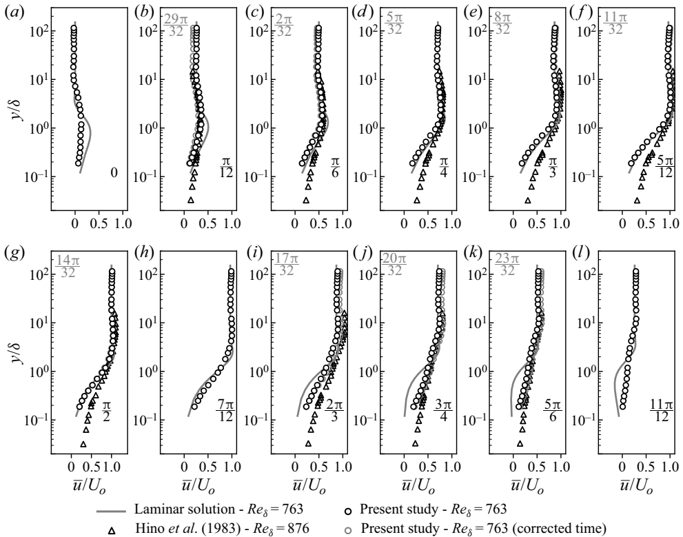
Figure 11. Ensemble-average velocity profiles \bar{u} normalized using the maximum velocity U_o for Re_\delta = 763 .
