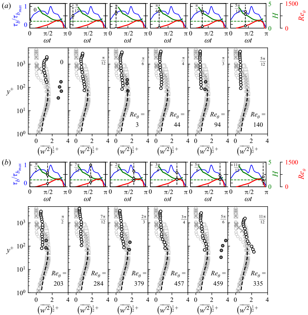
Figure 15. Ensemble-average spanwise r.m.s. profiles \sqrt{w^2}^+ for Re_\delta = 763 (the legend is the same as in figure 13).
