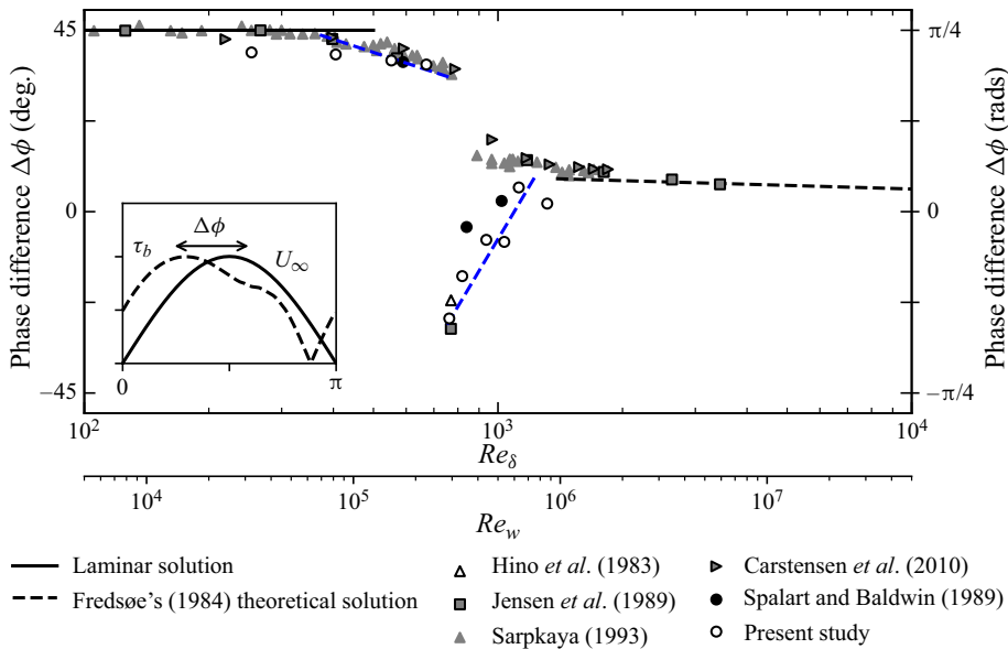
Figure 10. Phase difference \Delta\phi as a function of Re_\delta and Re_w .
