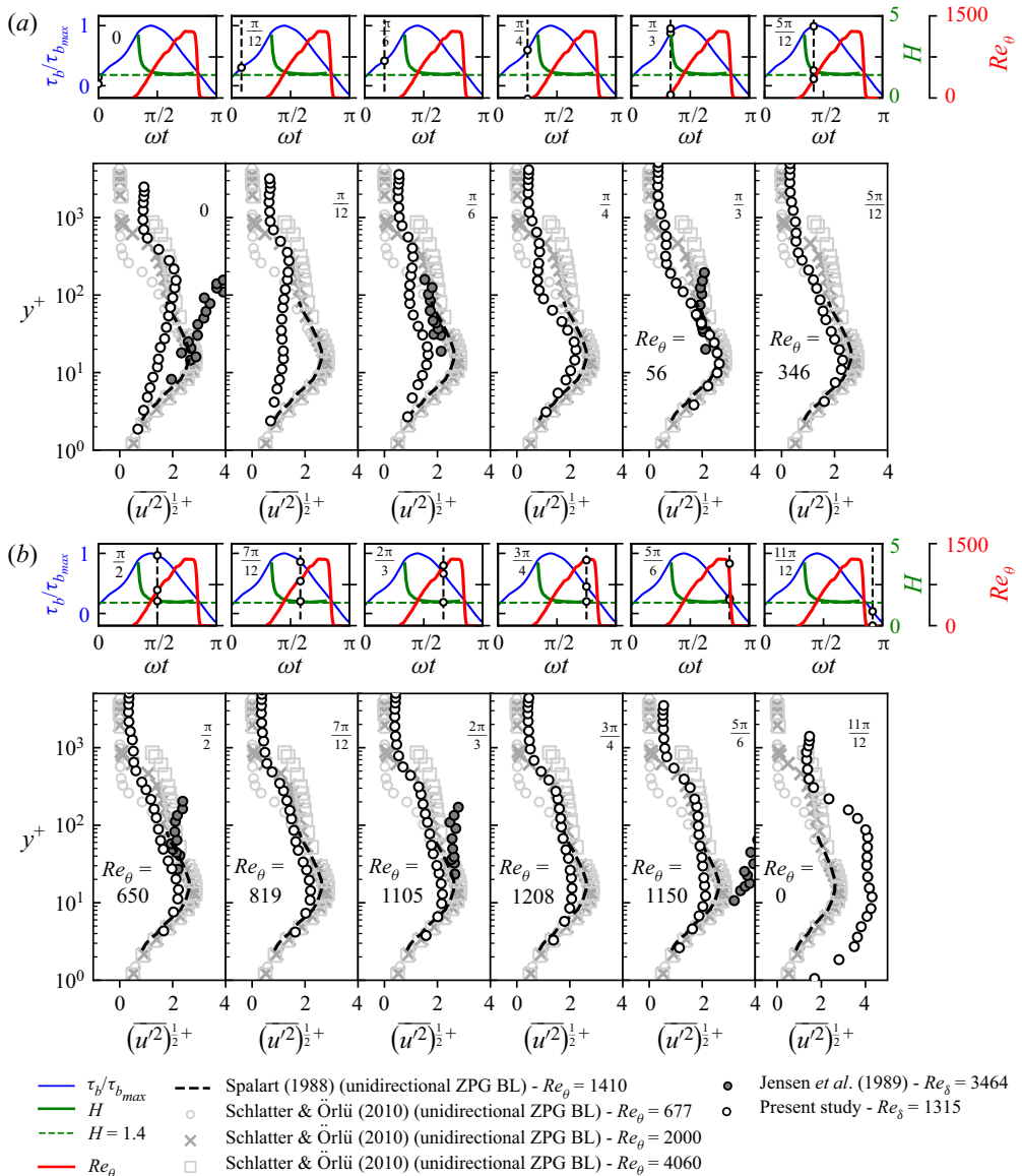
Figure 17. Ensemble-average streamwise r.m.s. velocity fluctuation profiles \sqrt{u^2}^+ for Re_\delta = 1315 .
