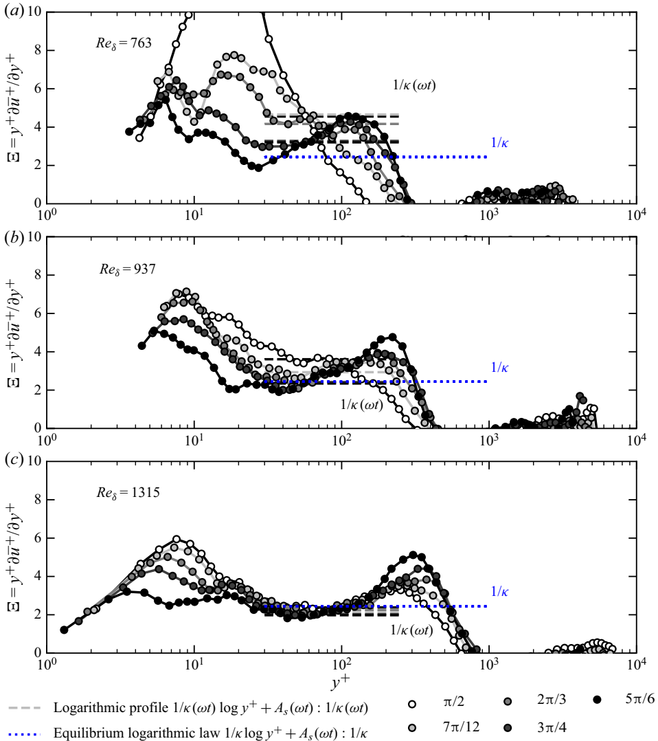
Figure 5. Log-law diagnostic function \mathcal{E} during the deceleration phase for Re_\delta values of 763, 937 and 1315.
