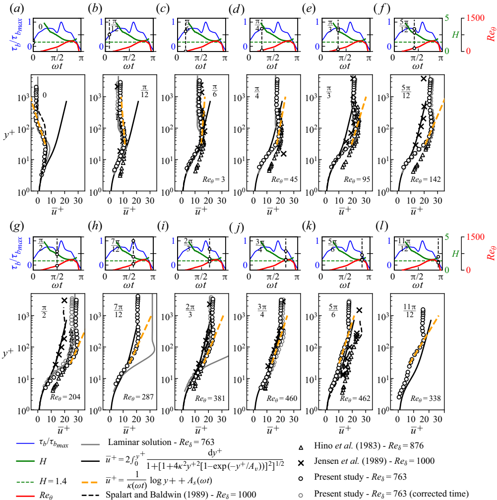
Figure 12. Ensemble-average velocity profiles \bar{u}^+ and logarithmic fit for Re_\delta = 763 . For comparison the equilibrium logarithmic law by VanDriest (1956) (where \kappa = 0.41 and A_v = 26 ) is also plotted.
