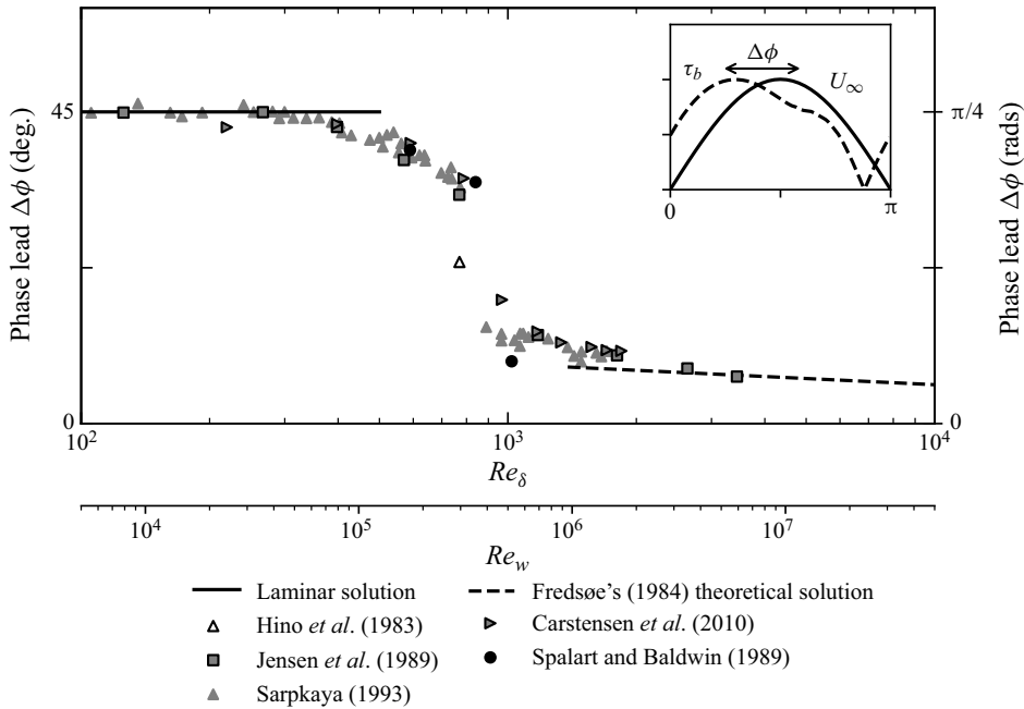
Figure 1. Typical phase lead \Delta\phi diagram as a function of Re_\delta and Re_w (adapted from Jensen et al. 1989).
