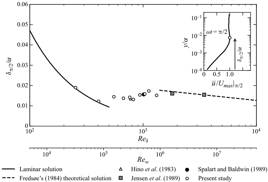
Figure 6. Normalized oscillatory boundary layer thickness \delta_{\pi/2}/\alpha as a function of Re_\delta or Re_w .
