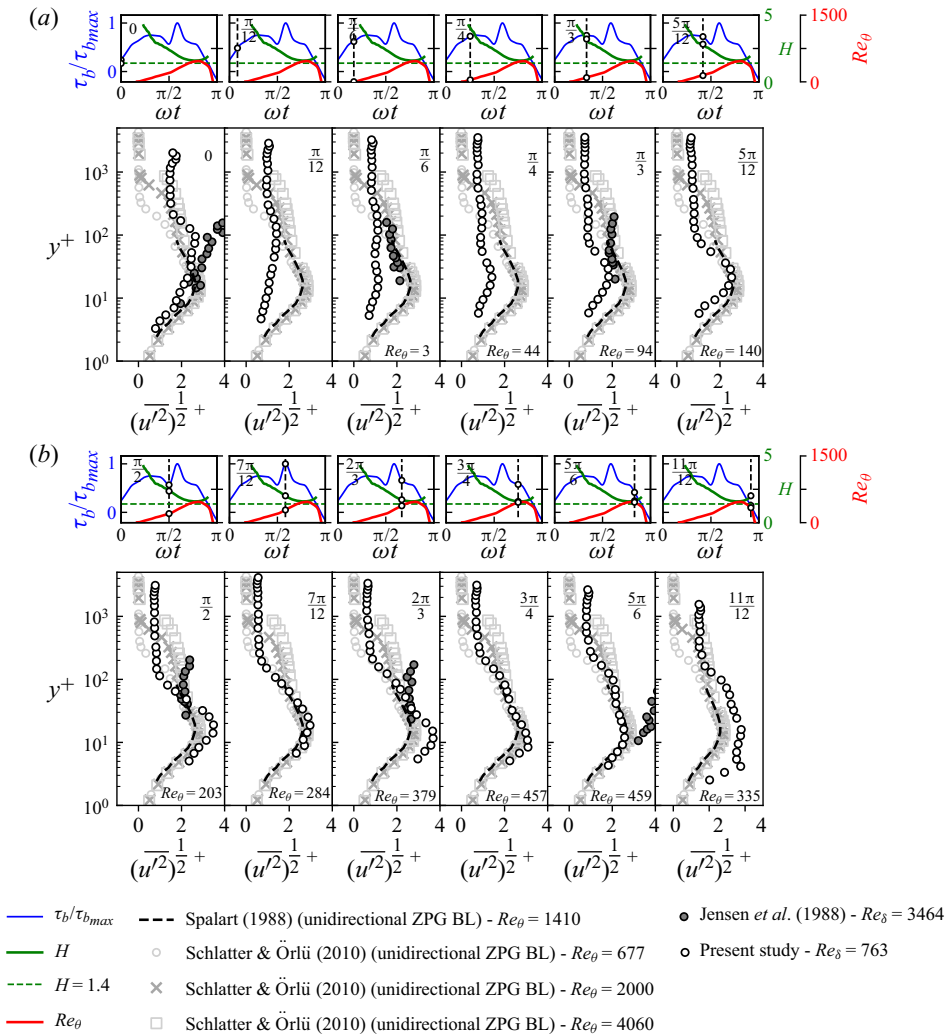
Figure 13. Ensemble-average streamwise r.m.s. profiles \sqrt{u'^2}^+ for Re_\delta = 763 .
