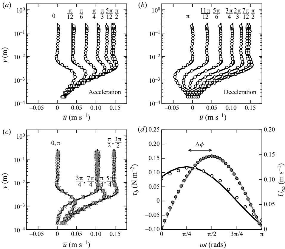
Figure 3. Comparison of measurements against analytical solution for laminar regime (Test 1, Re_\delta = 254 ): (a) streamwise velocity profiles during acceleration; \circ measurements, (—, black) analytical solution; (b) streamwise velocity profiles during deceleration; \circ measurements in the positive part, \times measurement in the negative part multiplied by -1.0 , (—, black) analytical solution; (c) comparison between positive and negative parts of the period, \circ measurements in the positive part, \times measurement in the negative part multiplied by -1.0 , (—, black) analytical solution; (d) measurements of bed shear stress \tau_b and free stream velocity U_\infty , \circ measurements of bed shear stress, ( \bullet , grey) measurements of free stream velocity, (—, black) analytical solution for bed shear stress \tau_b , --- U_\infty(t) = U_o \sin(\omega t) .
