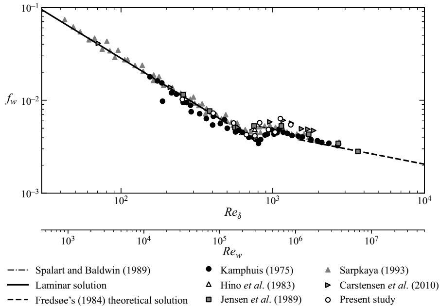
Figure 9. Friction factor f_w as a function of Re_\delta and Re_w .
