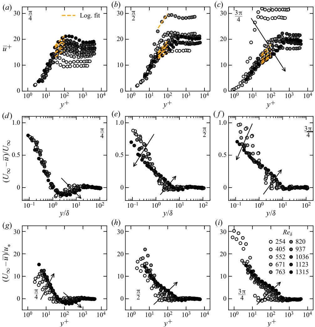
Figure 4. Reynolds number effect. Ensemble average velocity profiles in wall units for: (a) \omega t = \pi/4 ; (b) \omega t = \pi/2 ; (c) \omega t = 3\pi/4 . Ensemble average velocity defect profile normalized with free stream velocity U_\infty and \delta for: (d) \omega t = \pi/4 ; (e) \omega t = \pi/2 ; (f) \omega t = 3\pi/4 . Ensemble average velocity defect profile normalized with shear velocity u_* for: (g) \omega t = \pi/4 ; (h) \omega t = \pi/2 ; (i) \omega t = 3\pi/4 . Dashed orange lines show logarithmic fit for the cases with Re_\delta \geq 763 . The arrows show the increasing Re_\delta path.
