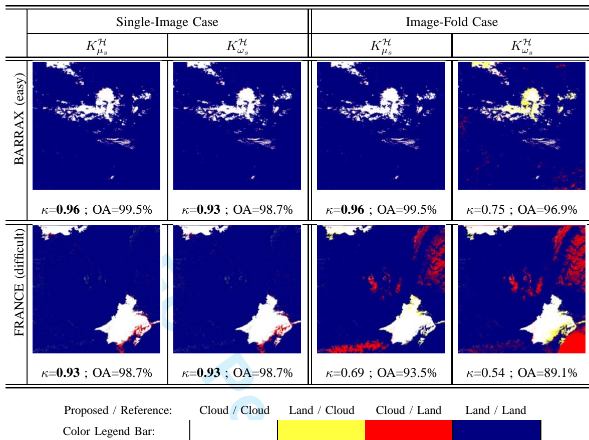
Fig. 5. Comparison of the cloud mask of kernel methods proposed against the reference cloud mask obtained from the user-driven unsupervised method proposed in [10] for the MERIS images over Barrax and France . Discrepancies between methods are shown in red when proposed kernel methods detect cloud and in yellow when pixels are classified as cloud-free.
