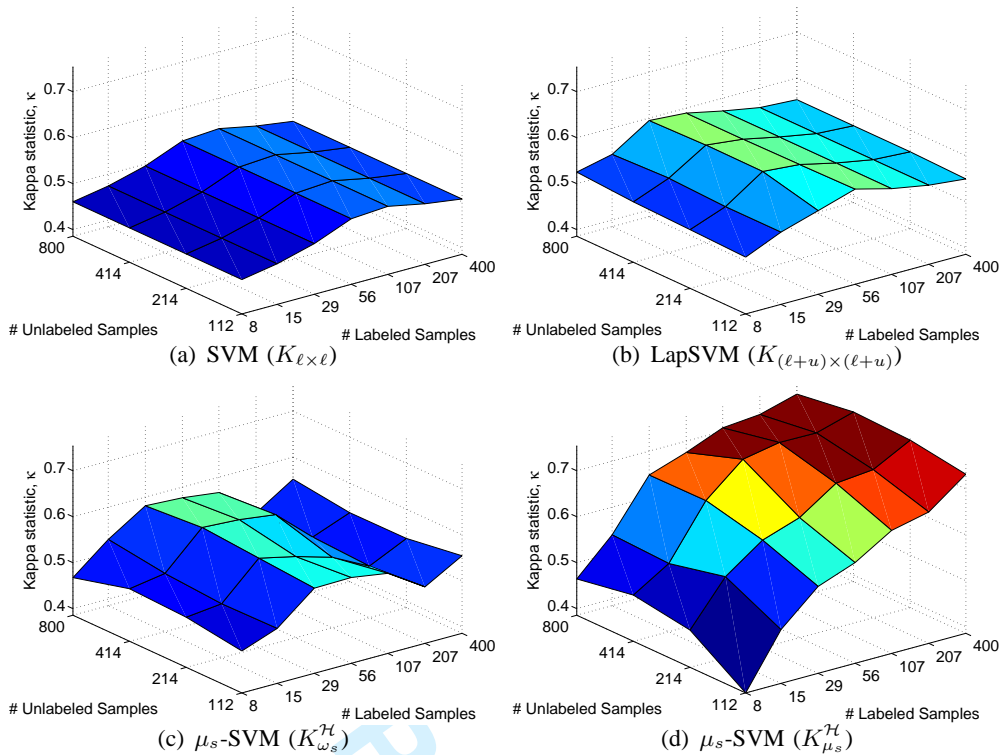
Fig. 6. Average cloud classification results for the 5 MERIS sample images (BR-2003-07-14, BR-2004-07-14, TU-2004-07-15, FR-2005-03-19, and FI-2005-02-26) training the model for each image with labeled samples from the other 4 images and unlabeled samples from the image to be classified ( image-fold case ): Kappa statistic surface over the validation set for the (a) SVM, (b) LapSVM, and \mu_s -SVM for (c) the K_{\omega_s}^H and (d) the K_{\mu_s}^H kernels as a function of the number of labeled ( \ell ) and unlabeled ( u ) samples.
