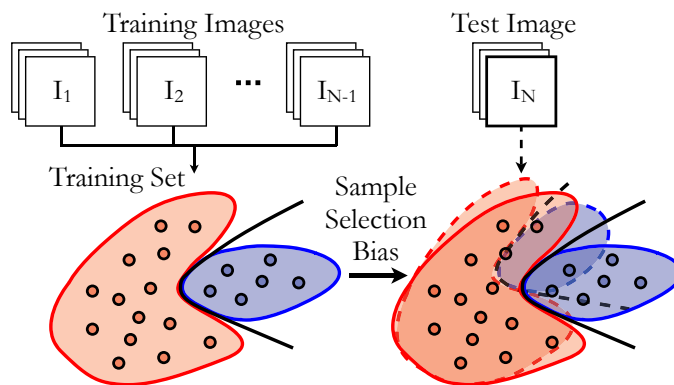
Fig. 1. Illustrative example of the sample selection bias produced when the distributions of training and test sets do not match, i.e. a good classifier in training fails when testing because of the distribution mismatch. This can be due to different reasons: the problem space is not adequately sampled, the extracted features for the training data do not closely represent test samples, or when labeled data are extracted from other images modeling similar problems. These are typical situations in remote sensing classification problems.
