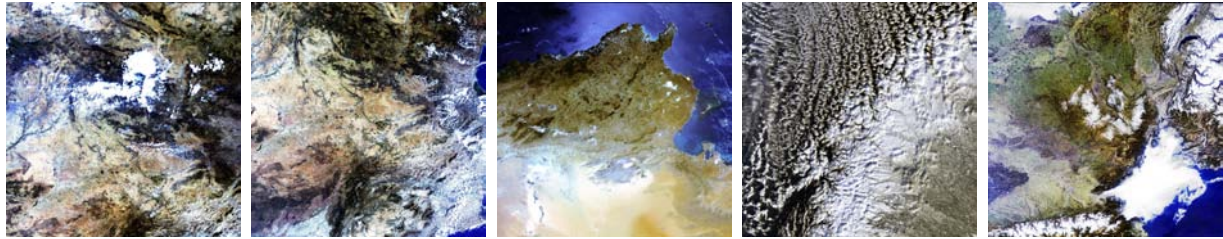
Fig. 3. MERIS images over Spain (BR-2003-07-14 and BR-2004-07-14), Tunisia (TU-2004-07-15), Finland (FI-2005-02-26), and France (FR-2005-03-19).
