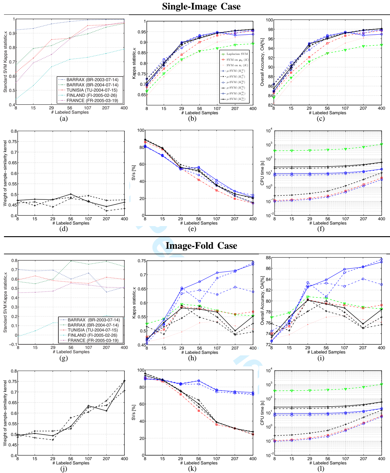
Fig. 4. Single-image case (a-f): Classification results training the models with labeled and unlabeled (800) samples from the image to be classified. Image-fold case (g-l): Classification results training the models with labeled samples from the other 4 images and 800 unlabeled samples from the image to be classified. Plots (a & g) show the standard SVM classification results ( \kappa ) for the 5 MERIS images and the other plots show average classification results over the 5 images: (b & h) \kappa , (c & i) OA [%], (d & j) weight \nu of the sample-similarity kernel of labeled samples K , (e & k) SVs [%], and (f & l) CPU time [s].
