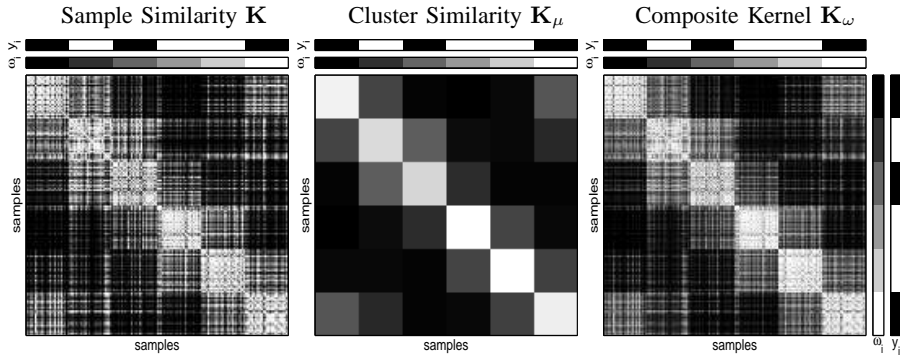
Fig. 2. Illustrative example of the three involved kernel matrices ( \ell \times \ell ): sample similarity accounted by the kernel of the training samples \mathbf{K} ( \nu = 1 ); cluster similarity accounted by the mean map kernel of the clusters \mathbf{K}_\mu ( \nu = 0 ); and the composite kernel \mathbf{K}_\omega obtained by combining the sample and the cluster similarities for each sample ( 0 < \nu < 1 ). Note that samples are sorted by class y_i and by cluster \omega_i for a proper interpretation.
