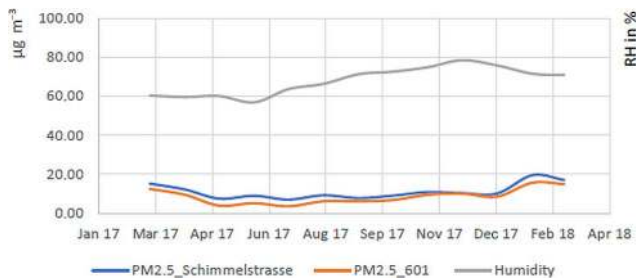
Figure 9. Monthly average PM and relative-humidity values for Schimmelstrasse.
