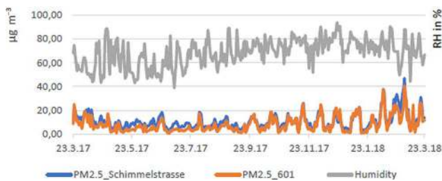
Figure 8. Daily average PM and relative-humidity values for Schimmelstrasse.
