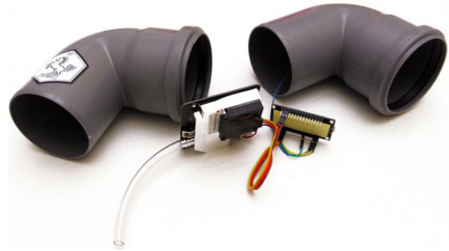
Figure 1. PM sensor kit.
