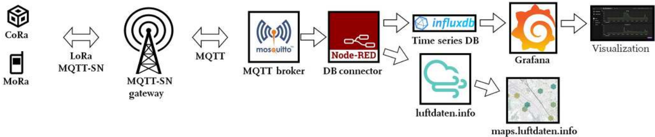
Figure 4. Sensing architecture.
