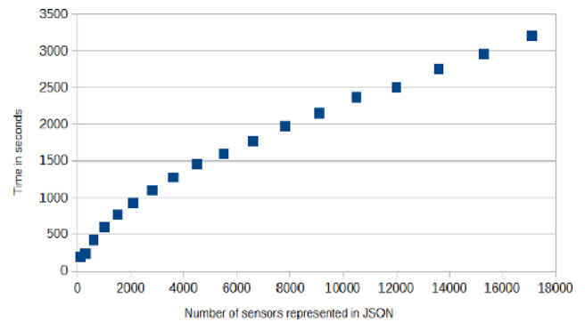
Figure 15. Time needed to create the RDF graph depending on the number of sensors.
