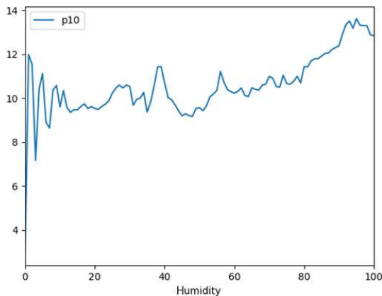
Figure 12. Median of PM_{10} against relative air humidity over 1 year.
