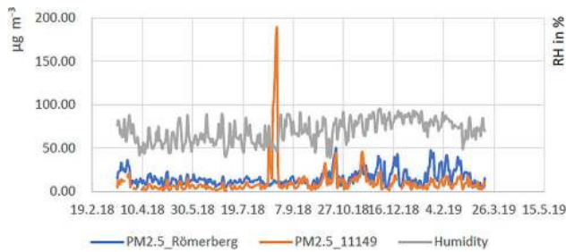
Figure 6. Daily average PM and relative-humidity values in Römerberg.
