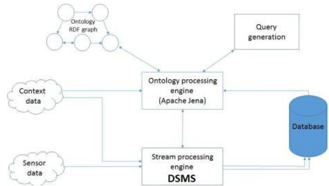
Figure 13. Architecture of the ontological population system.
