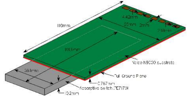
Fig. 2: Sketch of the mock-up handset including dimensions. Partly redrawn from [37].
