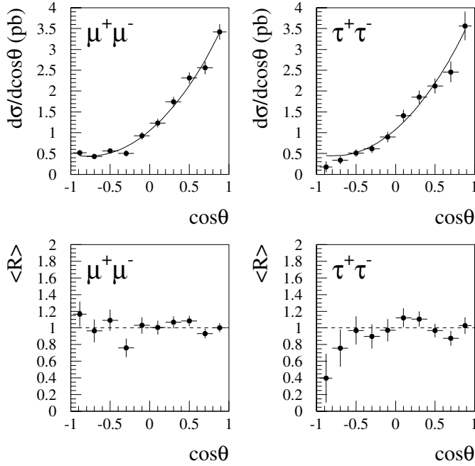
Fig. 12. Bin-by-bin averages, \langle R \rangle , for \mu^+\mu^- and \tau^+\tau^- final states. The lower plots show the values of \langle R \rangle while the upper plots show the SM d\sigma/d\cos\theta multiplied by \langle R \rangle at the luminosity weighted centre-of-mass energy for each measurement channel
