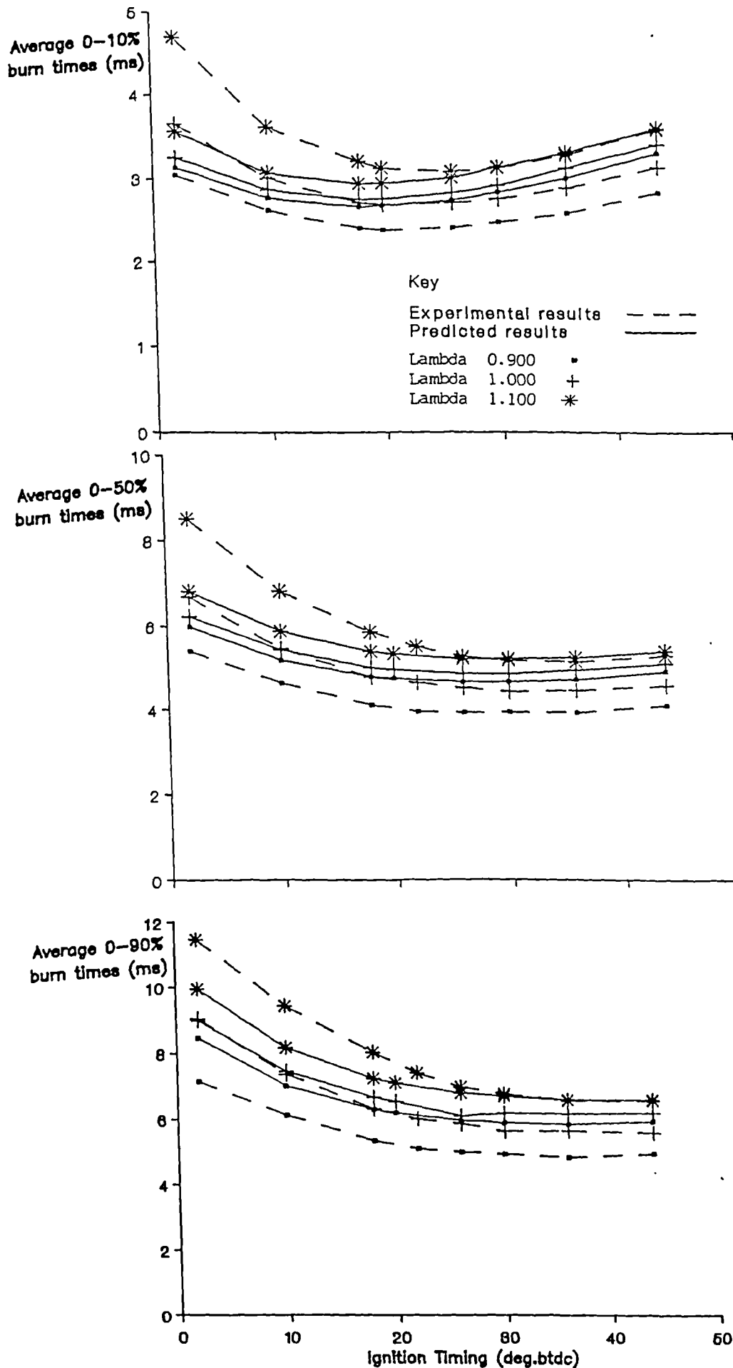
Figure 5.33: Comparison of experimental and predicted values for the variation of average burn times with ignition timing and mixture strength at part throttle.
