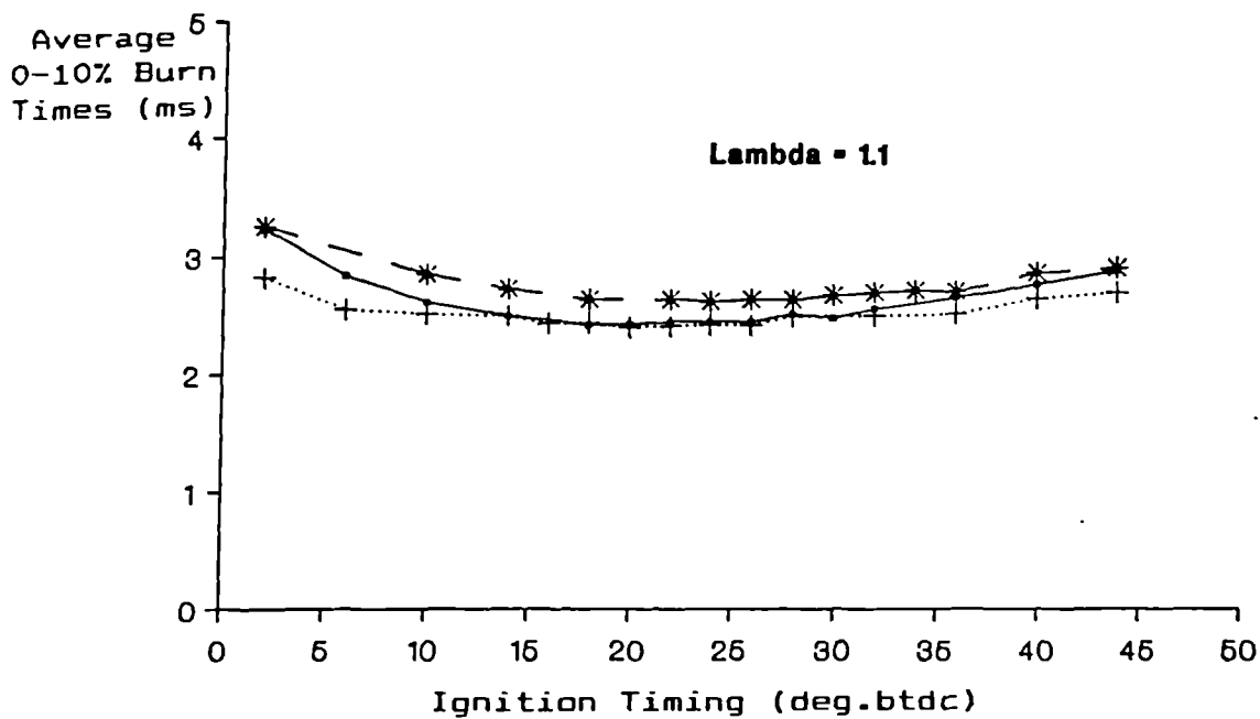
Figure 5.18: Average 0-10% burn times plotted on a lambda by lambda basis.
