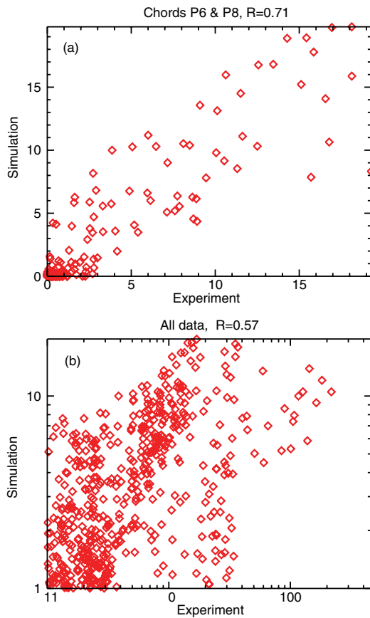
Figure 14. Calculated versus measured modulated signal. Both experimental and simulated spectra are averaged in 10 pixel-wide bins ( \sim 5 Å). Both axes are in arbitrary radiance units. (a) Sample correlation scatter plot showing good correlation when utilizing sightlines P6 & P8. This represents 6 spectra from 3 discharges. (b) The correlation for all 43 discharges (86 spectra) representing many experimental variations in density, temperature, magnetic field, elongation, plasma current, etc.
