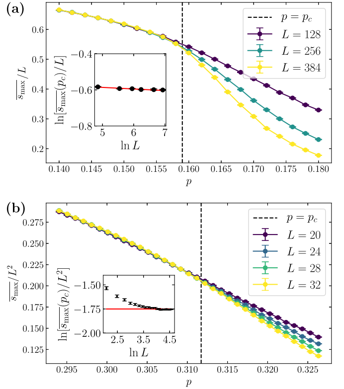
FIG. 11. The average size \overline{s_{\max}} of the largest entanglement cluster in the steady state for (a) 1 + 1D and (b) 2 + 1D Clifford circuits. The insets show log-log plots of this quantity at p = p_c , with the behavior well described by the power law \overline{s_{\max}}(p_c)/L^d \sim L^{-\beta_{ec}/\nu} , where \beta_{ec}/\nu = -0.009(2) for 1 + 1D and \beta_{ec}/\nu = 0.00(2) for 2 + 1D (power-law fits shown in solid red). Note there are strong finite-size effects in 2 + 1D, so there the fit is only to sizes L \geq 40 .
