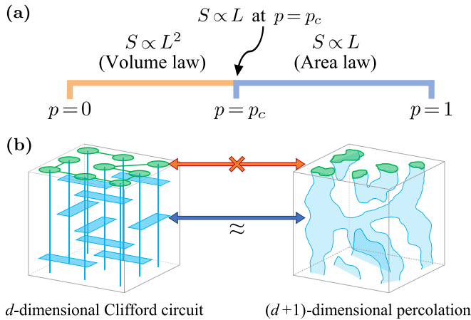
FIG. 1. (a) Phase diagram for the measurement-induced transition in 2 + 1D local random Clifford circuits. For measurement probabilities p < p_c the steady state exhibits volume-law entanglement, while for p \geq p_c the steady state is area-law entangled. The entanglement transition and the purification transition coincide. (b) The critical point of a d -dimensional circuit appears to be described by bulk exponents from the (d + 1)D percolation. However, entanglement cluster exponents do not match the percolation surface exponents.
