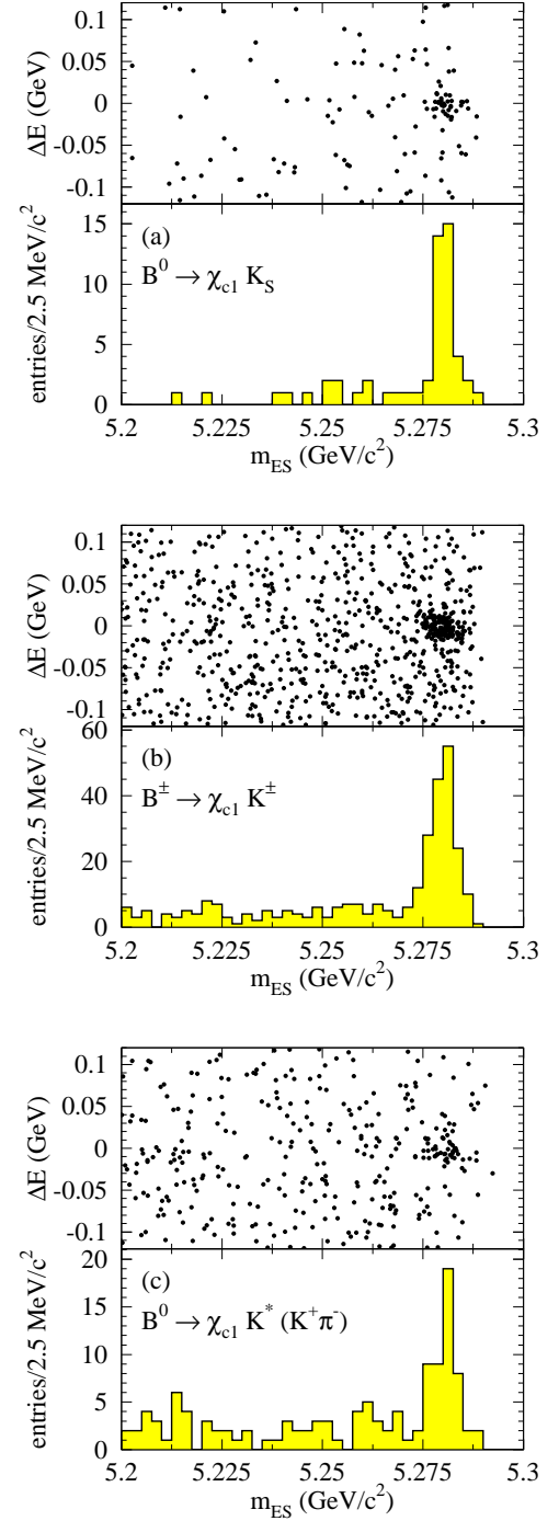
FIG. 12: Signal for (a) B^0 \rightarrow \chi_{c1} K_S^0 , (b) B^+ \rightarrow \chi_{c1} K^+ , and (c) B^0 \rightarrow \chi_{c1} K^{*0} (K^+ \pi^-) . The upper plots show the distribution of events in the \Delta E - m_{ES} plane, and the lower plots show the distribution in m_{ES} of events in the signal region in \Delta E .
