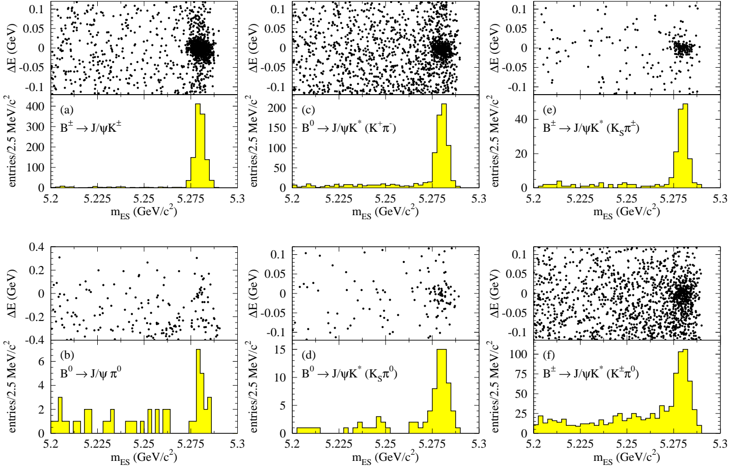
FIG. 10: Signal for (a) B^{\pm} \rightarrow J/\psi K^{\pm} , (b) B^0 \rightarrow J/\psi \pi^0 , (c-d) B^0 \rightarrow J/\psi K^{*0} , and (e-f) B^{\pm} \rightarrow J/\psi K^{*\pm} . The upper plots show the distribution of events in the \Delta E - m_{ES} plane, and the lower plots show the distribution in m_{ES} of events in the signal region in \Delta E .
